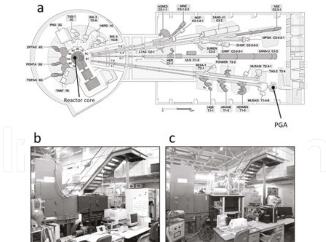
Figure 1. The location of PGA in JRR-3 (a). The PGA is at the end of the thermal neutron beam line (T1) in the guide hall. Two photographs taken in 2010 (b) and 2016 (c) show the difference before and after the automation upgrade. A revolute joint robot is set up at the side of the shielding body after the upgrade.
