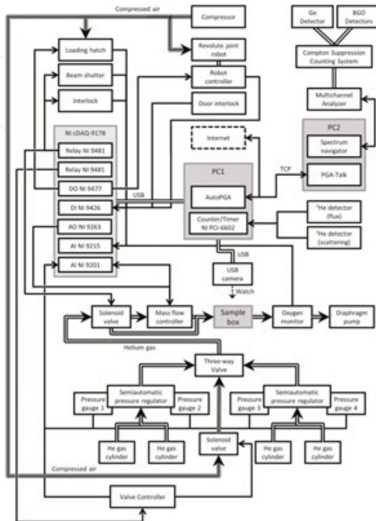
Figure 3. Connection diagram of the automated PGA system. The AutoPGA program installed in PC1 controls all the functions of the complex automation system and PC2 conducts prompt gamma-ray analysis using the existing measurement program and multichannel analyzer.
