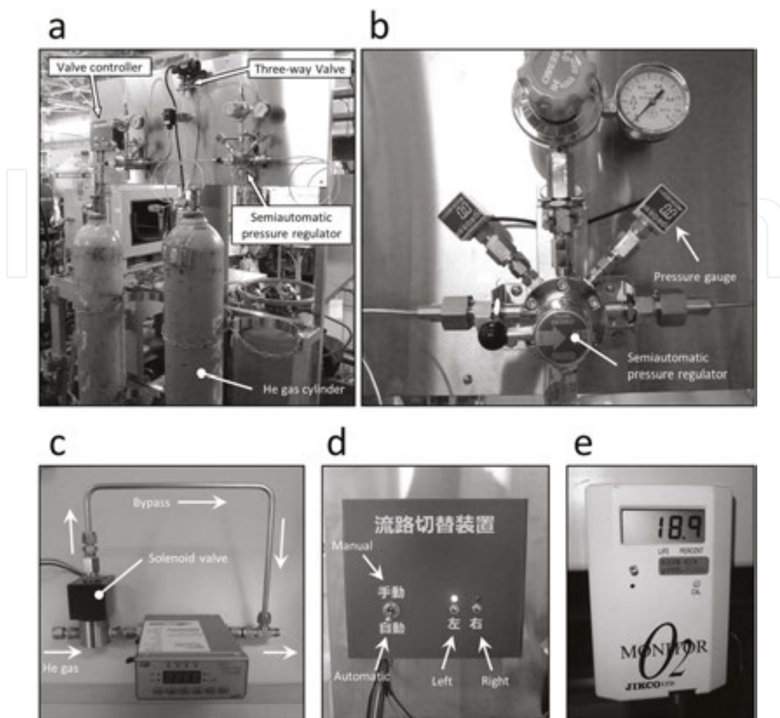
Figure 7. Equipment of the helium gas flow control system. Gas cylinder holder (a), pressure gauges connected with a semiautomatic pressure regulator (b), mass flow controller (c), valve controller (d), and oxygen monitor (e).
