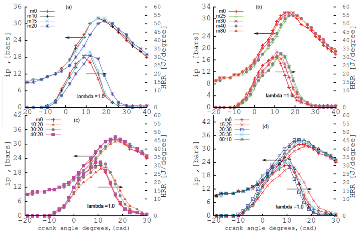
Figure 6. Effect of SAG (a, b) and DAG(c, d) blends on mean indicated pressure (IP) and heat release rate (HRR) at \lambda = 1.0 .
