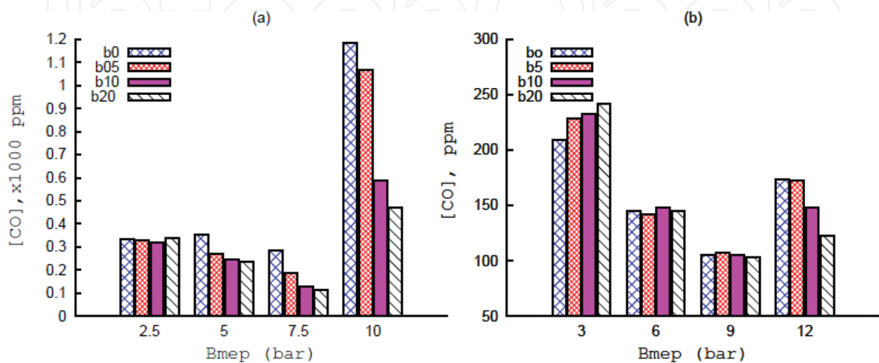
Figure 10. Carbon monoxide emissions (a) at 1500 rpm and (b) at 3000 rpm.
