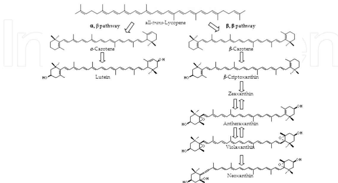
Figure 2. Biosynthetic pathway of carotenoids presents in the olive fruit.
