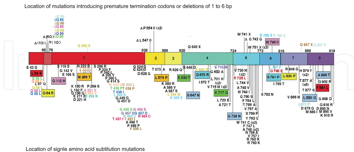
Figure 1. Schematic illustration of cataloged AR Somatic Mutations from the androgen receptor database. Mutations illustrated with the same color were present in the same cancer specimen. Mutations in red were found in the germline (image is courtesy of http://www.androgenbd.mcgill.ca , with permission from Dr. Mark Trifiro) [37].
