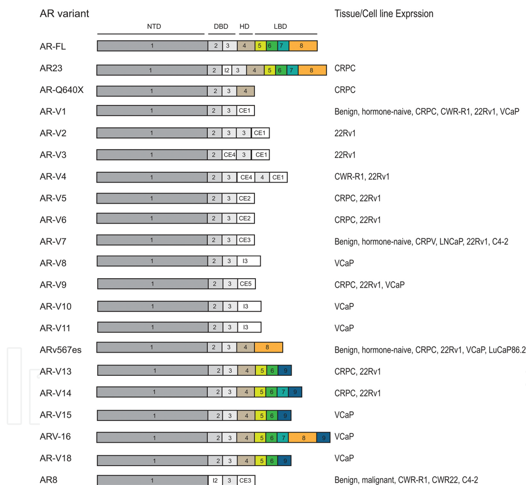
Figure 2. Schematic illustration of AR truncated and splice variants.
