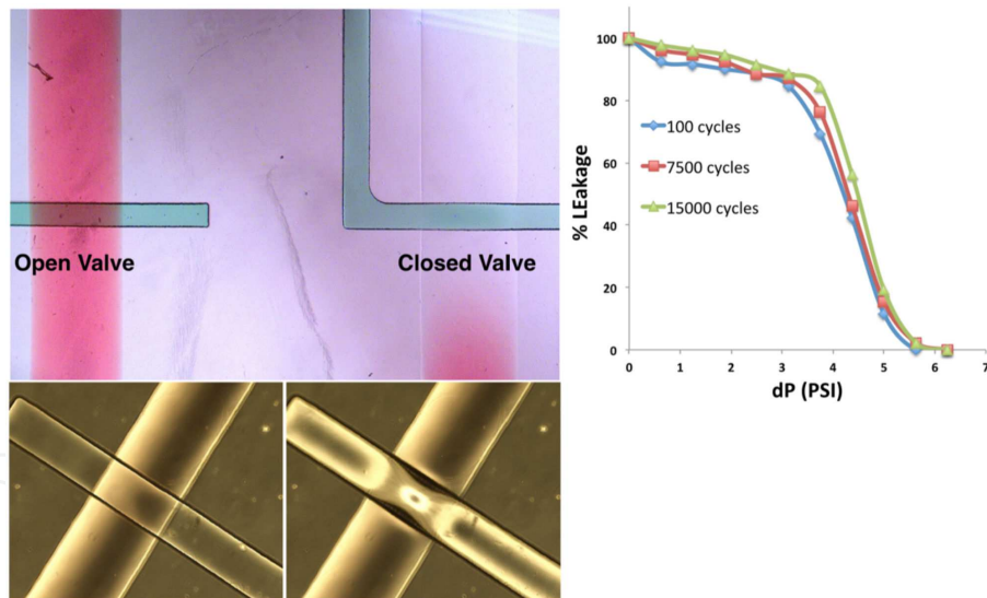
Figure 6. Valves evaluation and characterization. Valves were visualized using color dyes and inspected with a microscope inspection. Leakage was quantified after 100, 7500, and 15,000 switching cycles.
