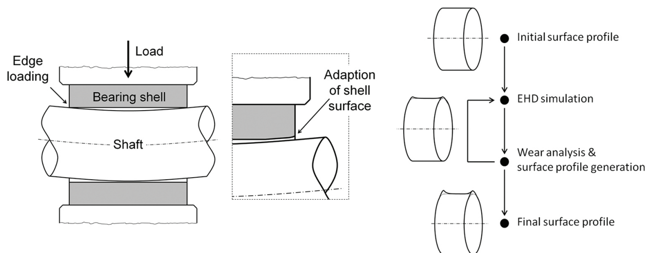
Figure 8. Edge loading caused by elastic bending of the shaft; the flowchart of the iterative surface profile generation on the right [42].
