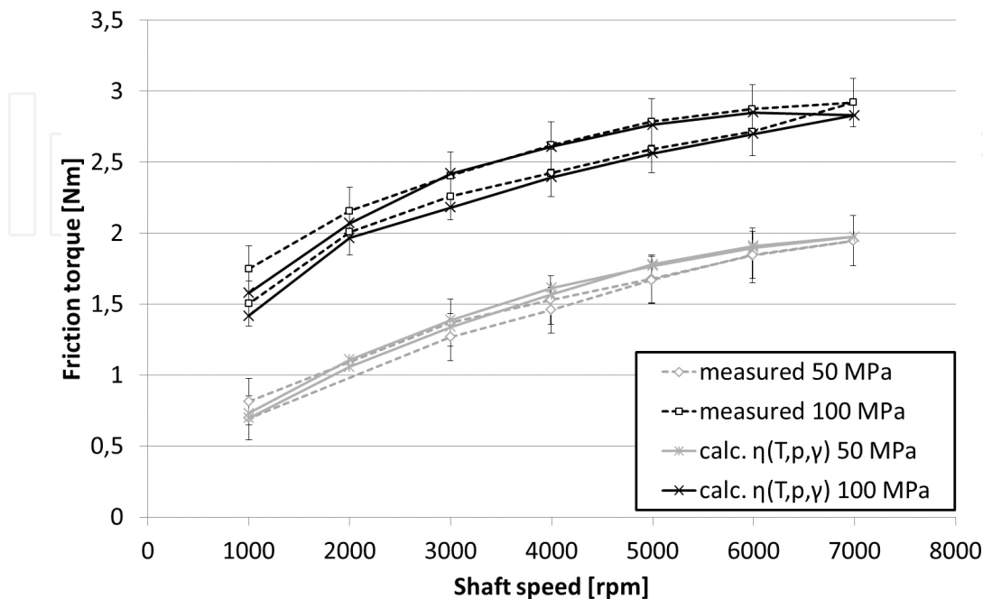
Figure 7. Comparison of the average friction torque measured on the test-rig with the simulated mean friction torque using the complete oil model \eta(T,p,\gamma;) at 50 and 100 MPa specific loads [47].
