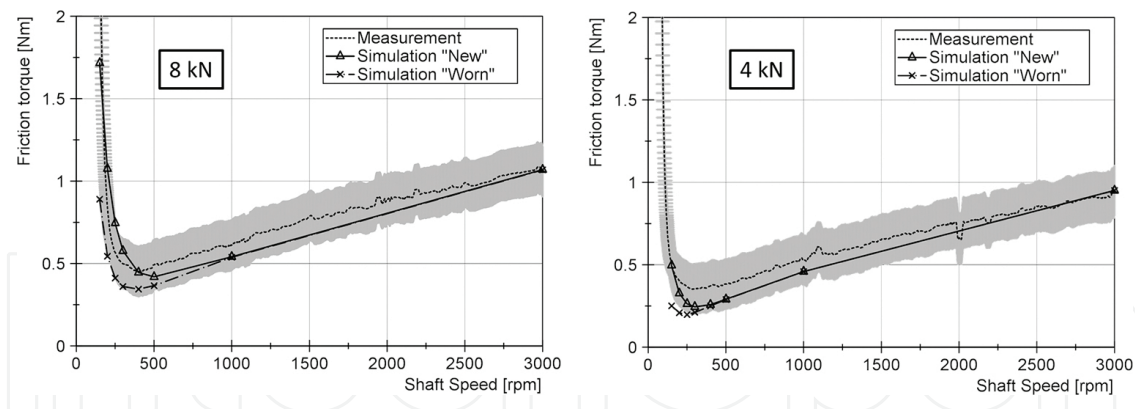
Figure 13. Comparison between the calculated and measured friction torque over shaft speed at a load of 8 and 4 kN [43].
