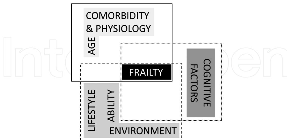
Figure 1. Venn diagram showing the overlap of different domains, all of which contribute to the eventual development and progression of frailty.
