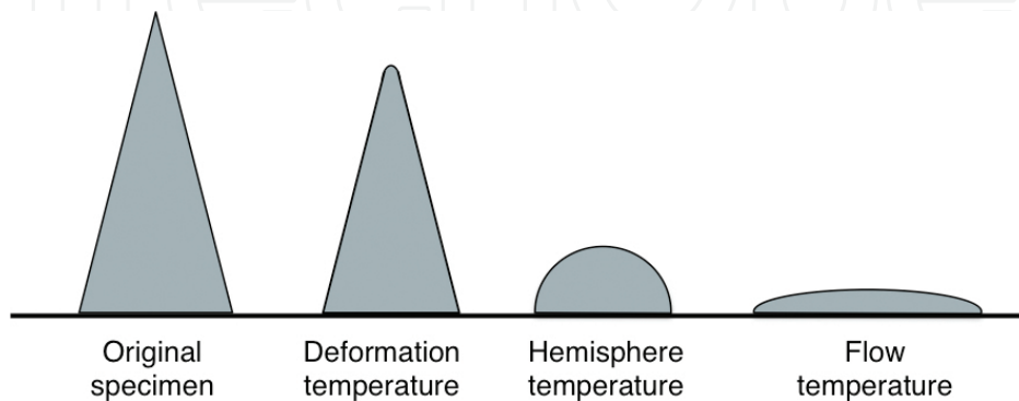
Figure 7. Ash characteristic temperatures.
