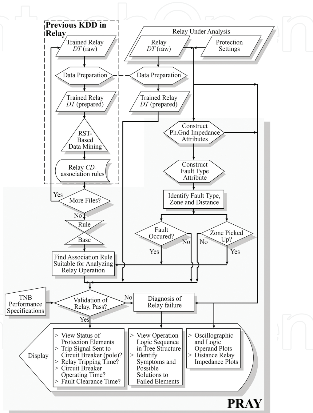
Figure 5. Architecture of Protective Relay Analysis System (PRAY).
