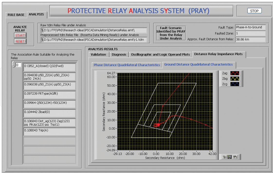
Figure 8. GUI for ground distance quadrilateral characteristics plots.
