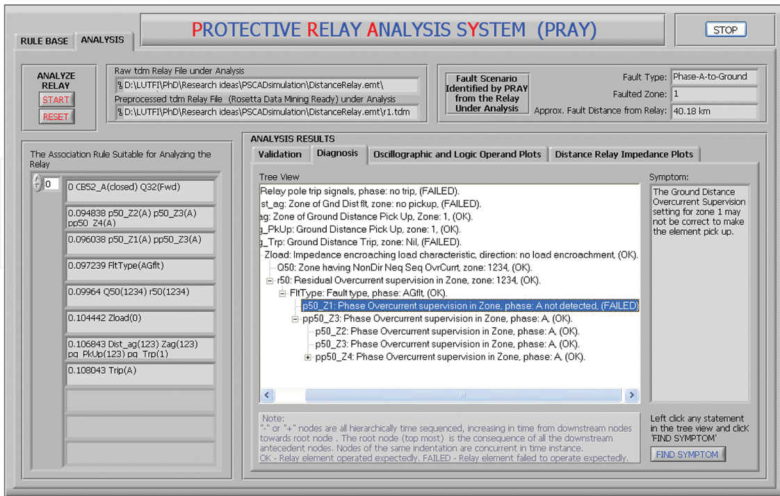
Figure 10. Diagnosis of misoperative relay.
