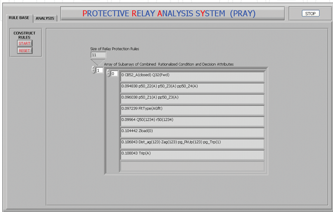
Figure 6. GUI for constructed rule base.
