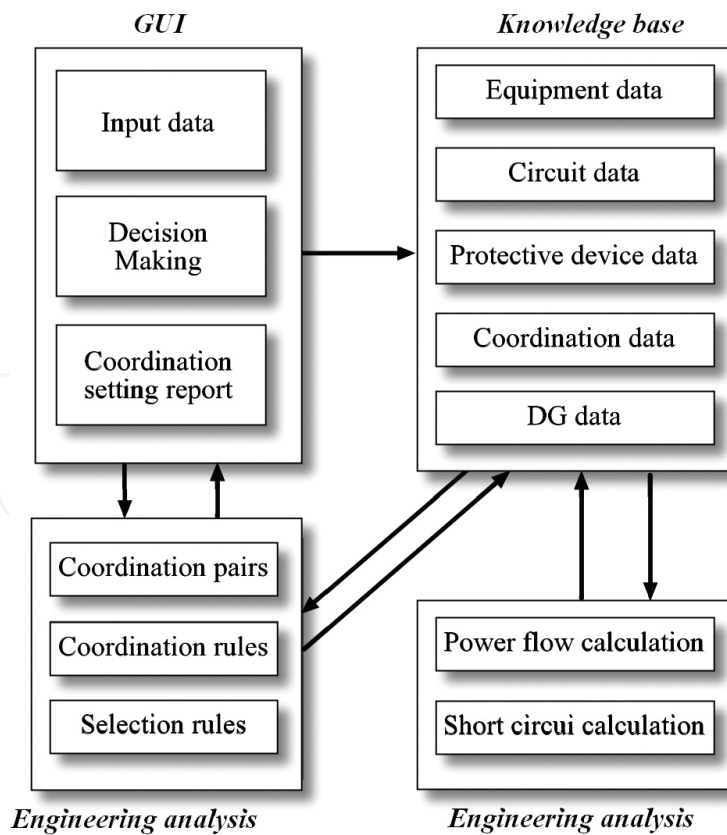
Figure 3. Structure of Expert System for protection coordination [13].
