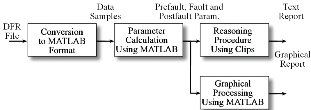
Figure 1. The Expert System block diagram [6].
