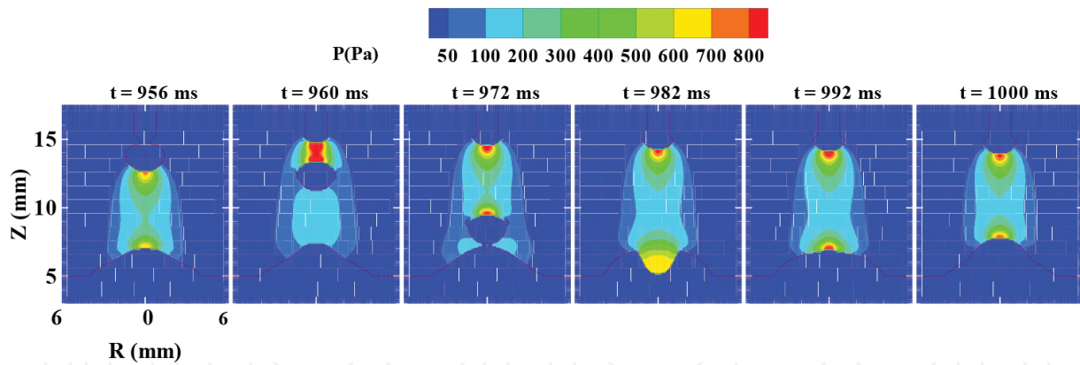
Figure 13. Pressure distributions in the arc plasma during the last droplet impingement and weld-pool dynamics.
