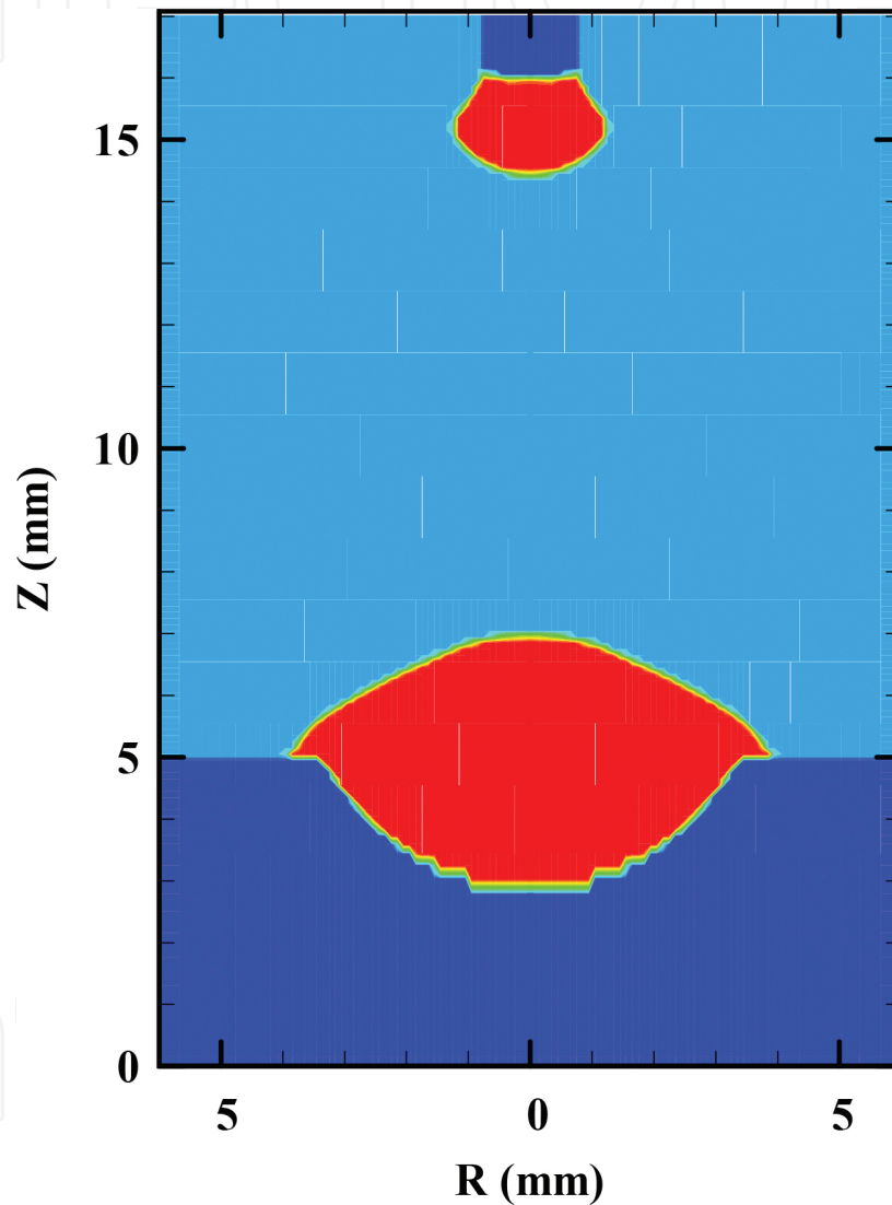
Figure 14. The solidified weld-bead shape.
