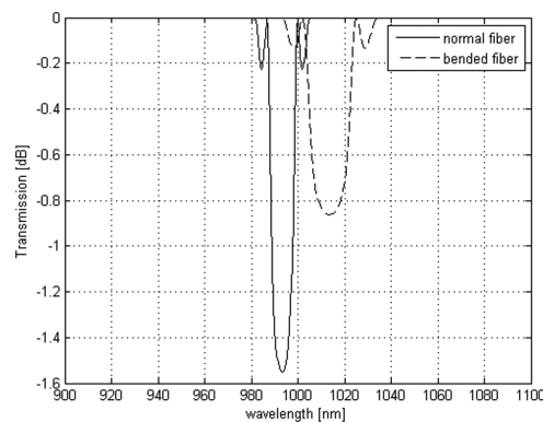
Figure 11. LPG transmission spectra simulated for a bent optic fiber in normal state. LPG period = 400 \mu\text{m} , LPG length L = 75 mm, grating amplitude \Delta n_{\text{eff}} = 25e-4 .
