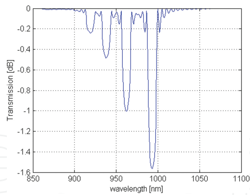
Figure 10. LPG transmission spectra simulated for an optic fiber in normal state. LPG period = 400 \mu\text{m} , LPG length L = 75 mm, grating amplitude \Delta n_{\text{eff}} = 25e-4 .
