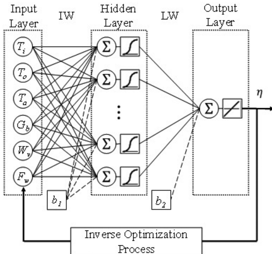
Figure 8. Inverse artificial neural network.
