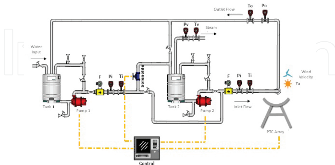
Figure 1. Operation diagram of parabolic solar concentration experimental system.
