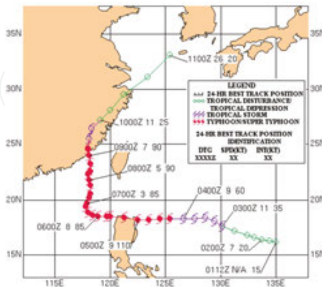
Figure 2. Best track of Typhoon Dan (1999) from the JTWC (adapted from Ref. [7]).
