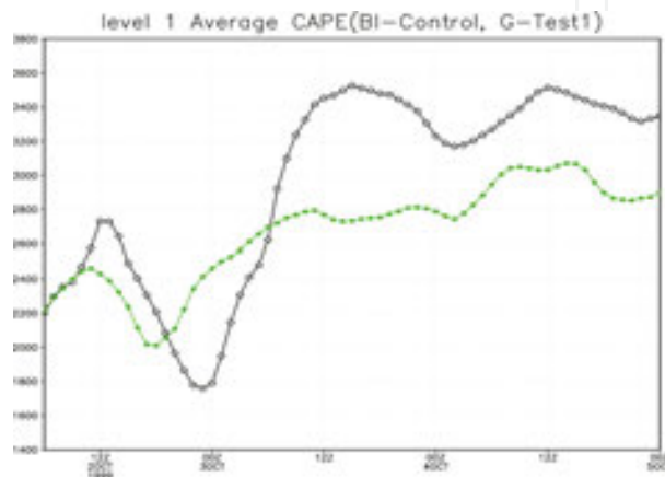
Figure 18. Area-averaged (13–17°N, 127–132°E) surface-based CAPE during formation of Typhoon Dan in the control WRF experiment (black) and sensitivity test (green).
