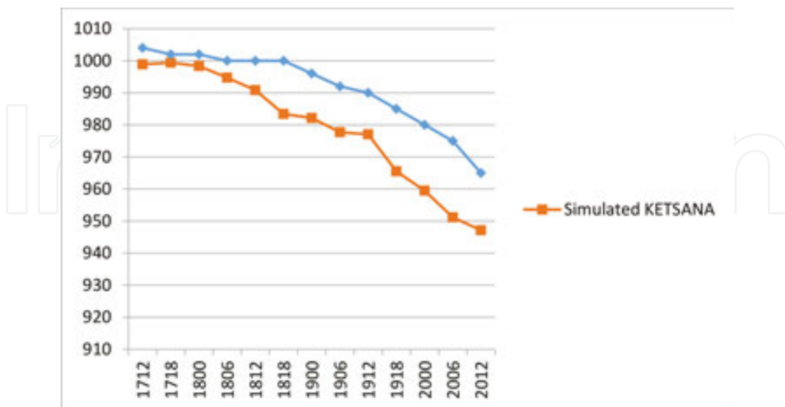
Figure 9. Simulated (red) and JMA best-track minimum surface pressure (hPa) of Typhoon Ketsana during 0000 UTC, October 17–20, 2003.
