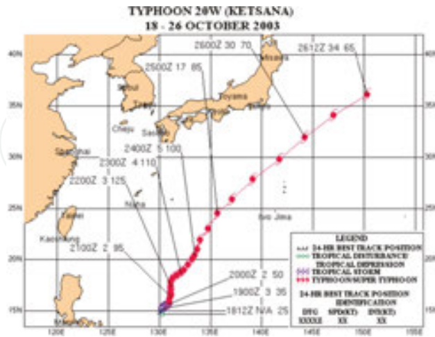
Figure 1. Best track of Typhoon Ketsana (2003) from the JTWC (adapted from Ref. [6]).
