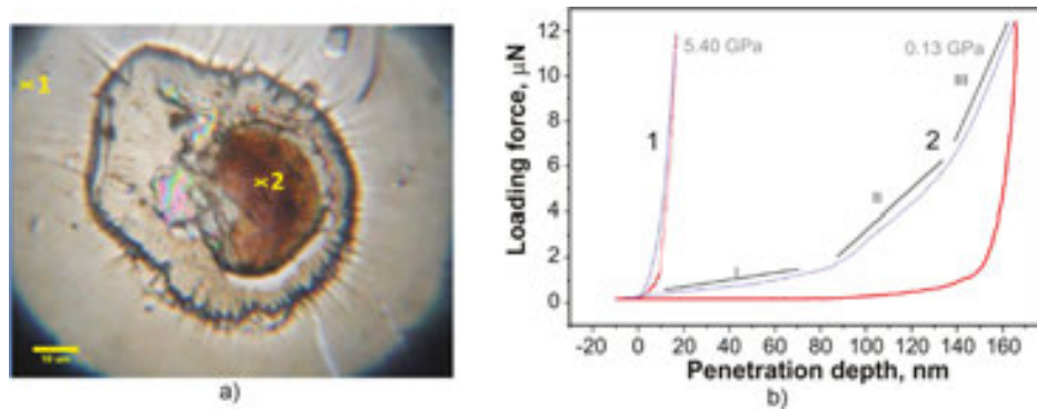
Figure 28. (a) Location of pricks by a nano-pin (yellow crosses) at the surface of a large dome-like blister, seen in Figure 23a . (b) The load and unloading curves of indenter measured at locations indicated in (a).
