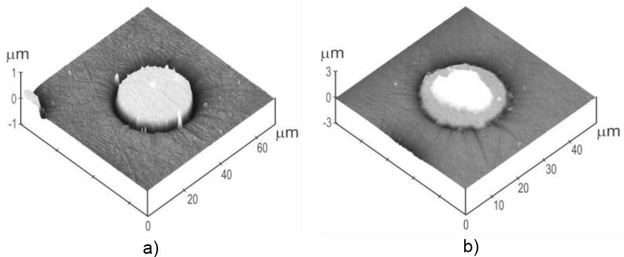
Figure 24. The AFM images of two different kinds of blisters: (a) with flat lid and (b) with a dome-like lid [26].
