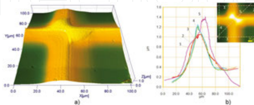
Figure 16. AFM data for the same sample of grade #3 exposed to plasma through Ni gauze as in Figure 15 : (a) 3-D picture near crossing of Ni wires, (b) 2D picture of same data and height distributions along the lines shown in picture.
