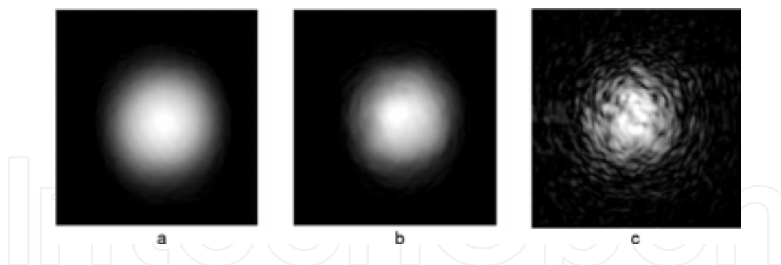
Figure 21. Image of the Ne-He laser beam spot after the beam was reflected from (a) “ideal mirror”, (b) from sample of grade #2 after sputtering 13.4 \mu\text{m} , and (c) from crystallized sample of grade #2 after sputtering 8.9 \mu\text{m} [24].
