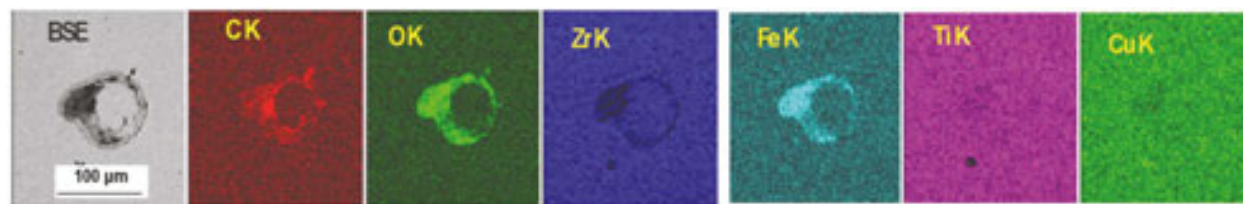
Figure 26. EDX-maps for a part of #1 sample surface with a large blister ( \sim\text{Ø}65\ \mu\text{m} ).
