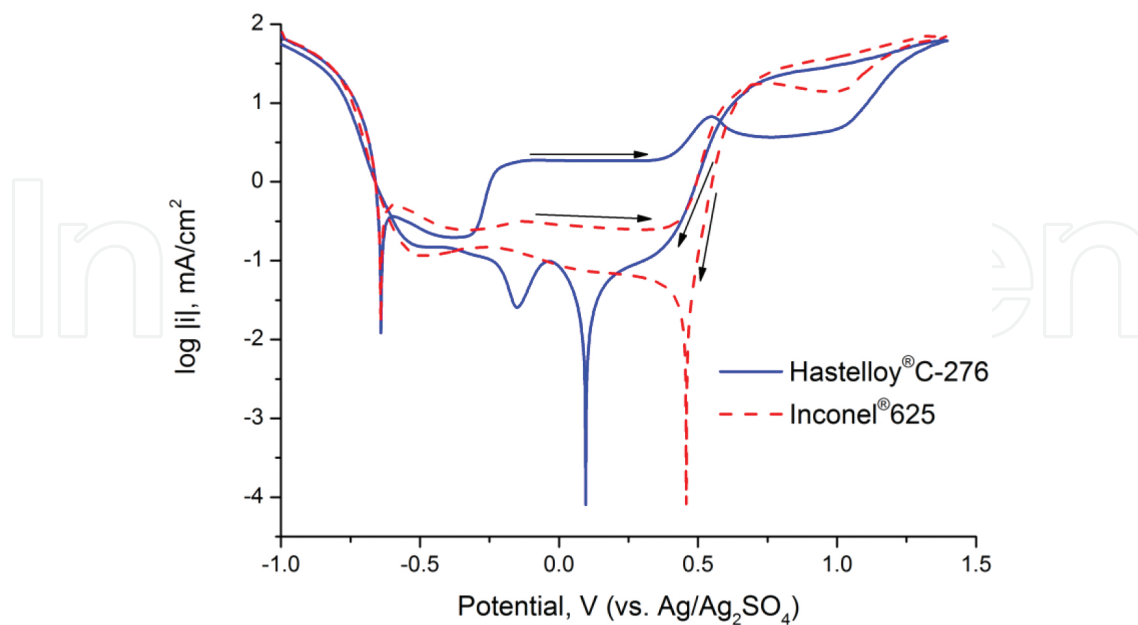
Figure 8. Polarization curves for Hastelloy ® C-276 and Inconel ® 625 wires in molten \text{KH}_2\text{PO}_4/\text{K}_2\text{H}_2\text{P}_2\text{O}_7 at 260^\circ\text{C} . Scan rate 1 mV/s.
