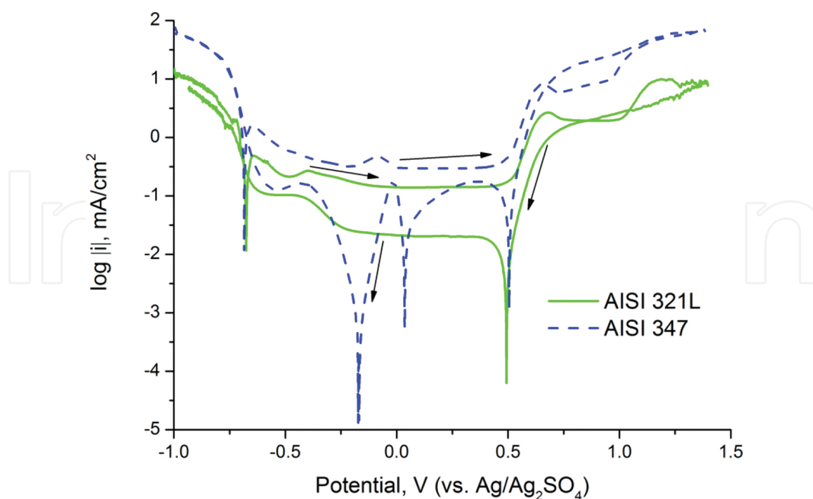
Figure 7. Polarization curves for AISI 321L and AISI 347 wires in molten \text{KH}_2\text{PO}_4/\text{K}_2\text{H}_2\text{P}_2\text{O}_7 at 260^\circ\text{C} . Scan rate 1 mV/s.
