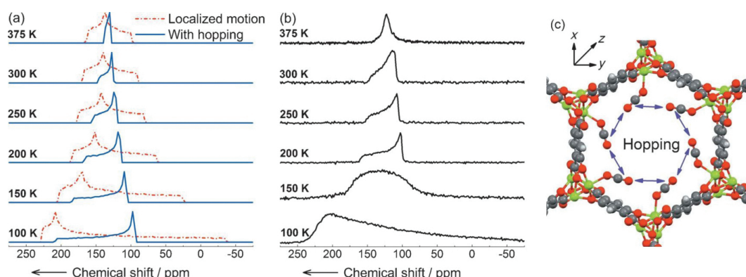
Figure 8. Studying dynamics of 13 CO 2 molecules adsorbed into Mg-MOF-74. (a) and (b) The comparison between the simulated and the measured static 13 C NMR spectra, which show lines broadened by chemical shift anisotropy. The comparison indicates that at about 100 K CO 2 molecules undergo localized motion around the minimum-energy positions, whereas at 200 K and above motion includes hopping of molecules between different metal sites, as indicated in (c). Figures were published by Lin et al. [39]. Copyright © 2013 Wiley-VCH.
