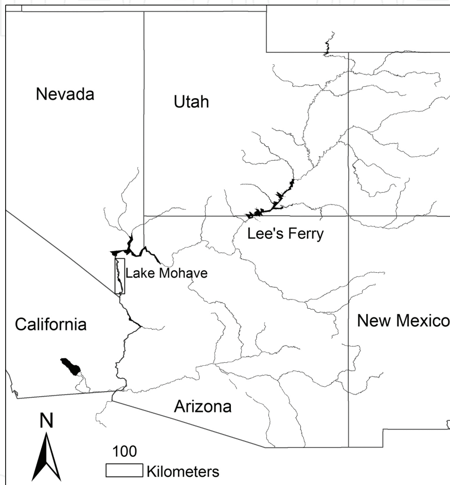
Figure 1. Map of the Colorado River drainage in western USA.
