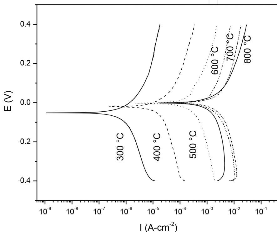
Figure 6. Tafel plots of Pt-YSZ at 300–800°C.
