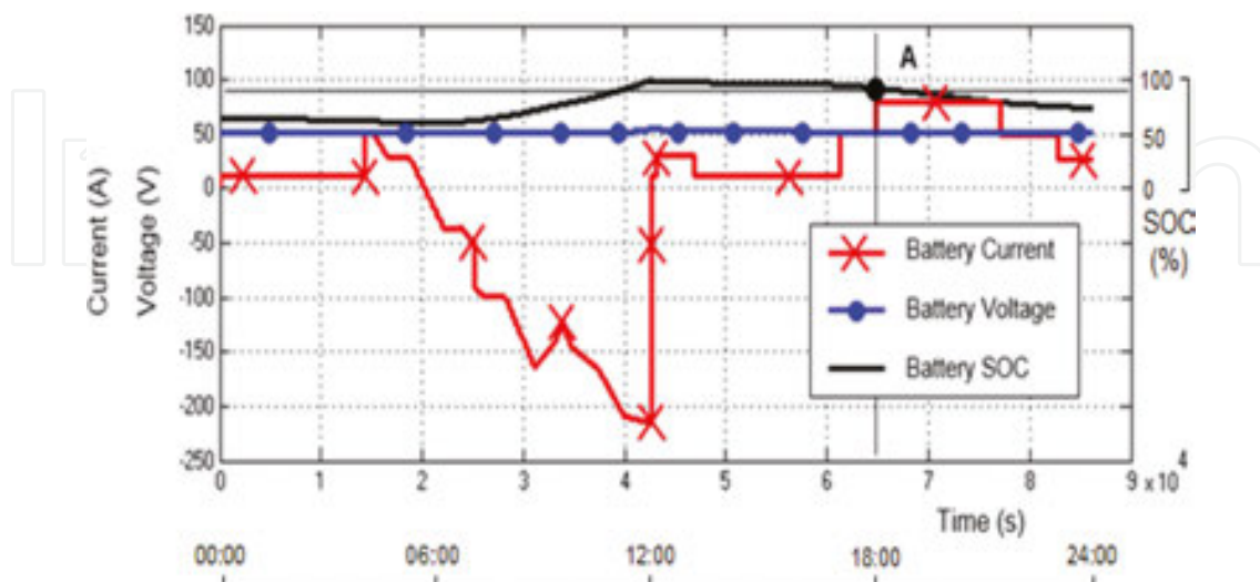
Figure 9. Scenario B: battery status.
