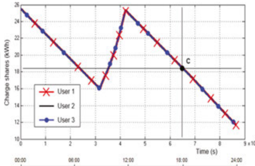
Figure 8. Scenario A: energy allocation.
