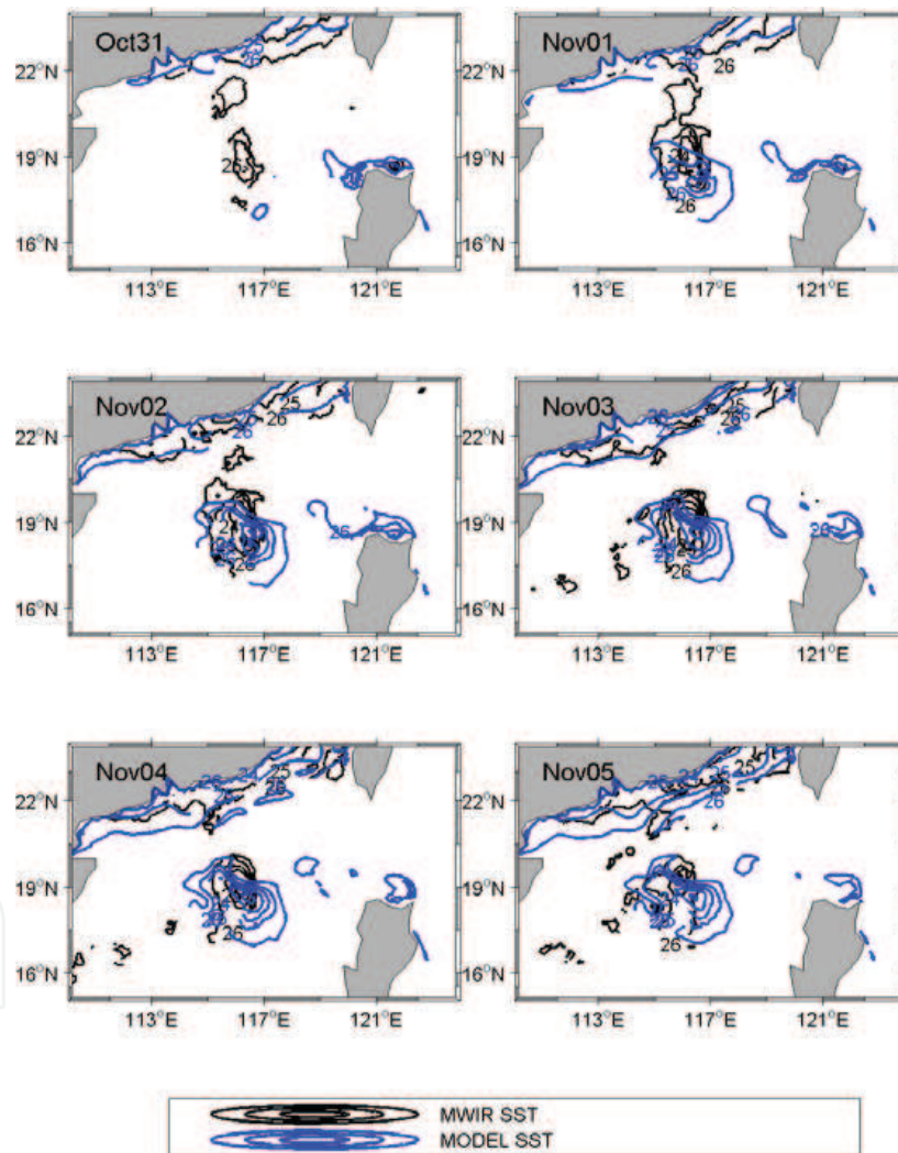
Figure 4. Isotherms of SST in the typhoon wake (unit: °C) from October 31 to November 5, 2006 (with the black lines showing the MWIR OI SSTs and blue lines showing the simulated SSTs).
