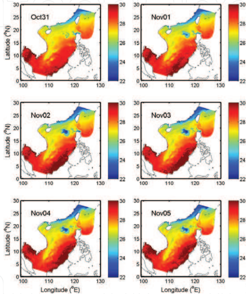
Figure 2. The simulated SSTs (unit: ^{\circ}\text{C} ) from October 31 to November 5, 2006.
