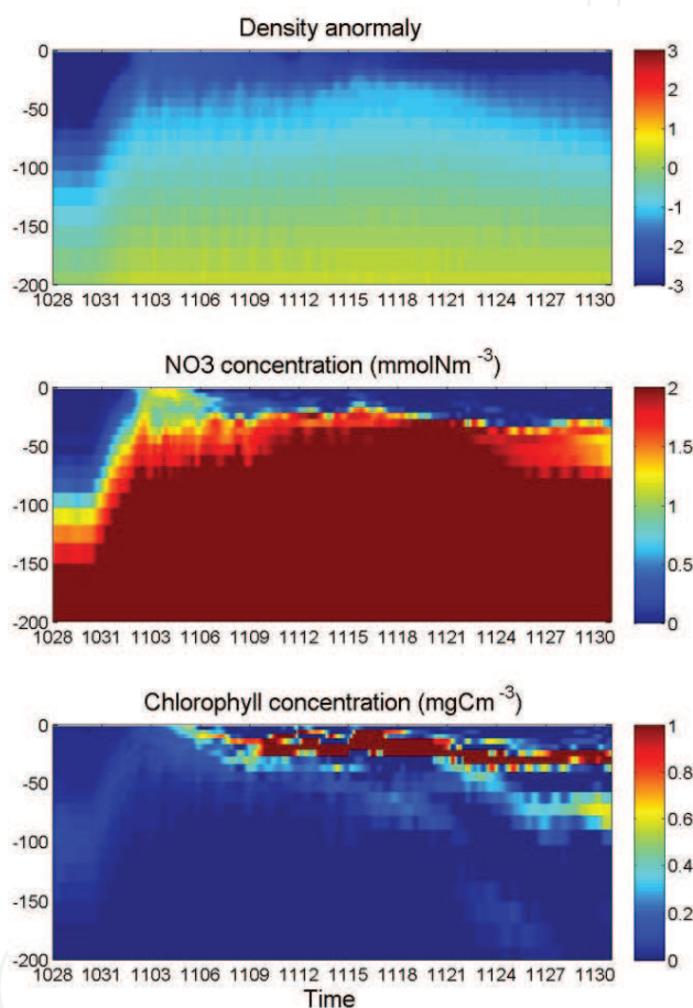
Figure 9. Profiles of chlorophyll a and nitrate concentration at the location ( 18.66^{\circ}\text{N} , 115.89^{\circ}\text{E} ), shown in Figure 7 in the typhoon wake from October 28 to November 30, 2006.
