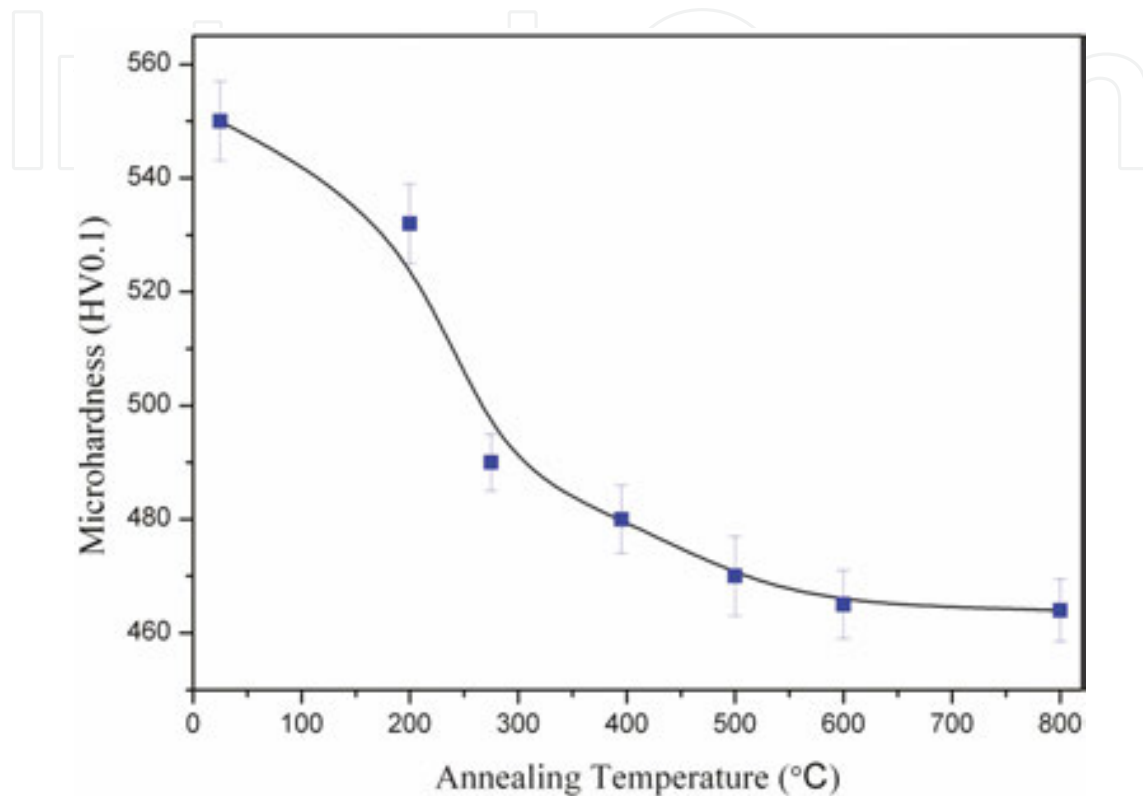
Figure 8. The change in Vickers microhardness values for \text{Cu}_{50}\text{Zr}_{40}\text{Ni}_5\text{Al}_5 alloy prepared by the wheel speed of 35 \text{ ms}^{-1} with annealing temperatures.
