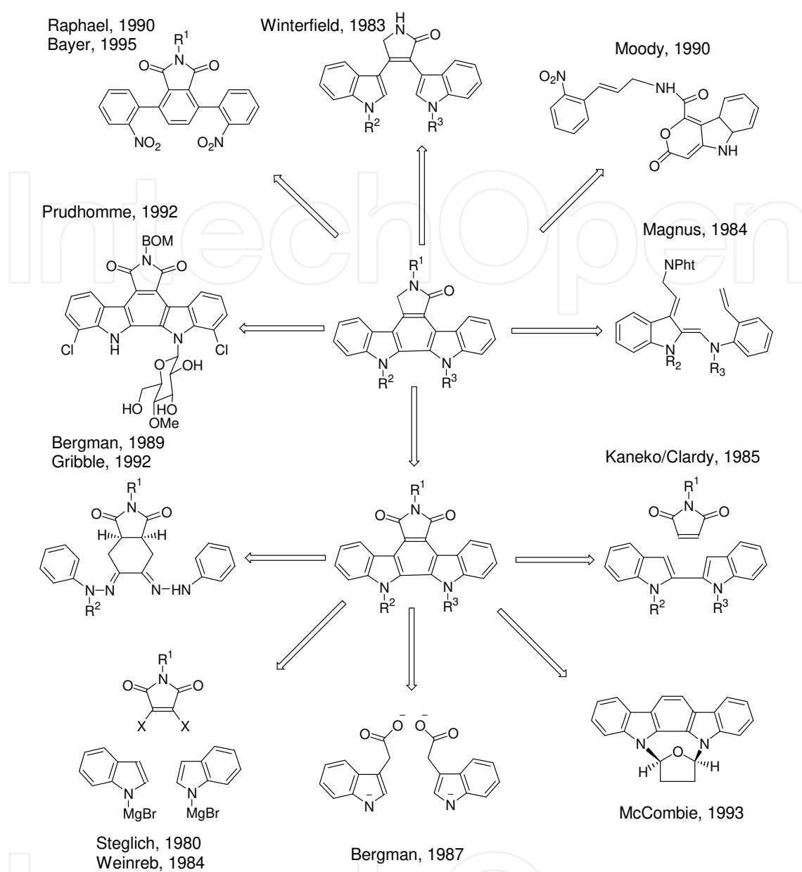
Figure 2. Approaches to indolocarbazole alkaloids
