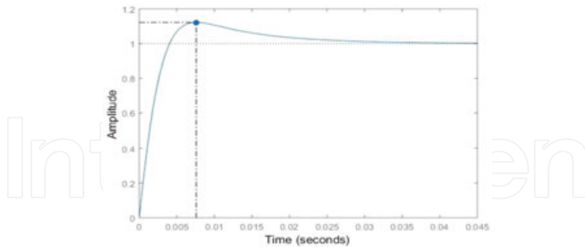
Figure 22. Time response of the system.
