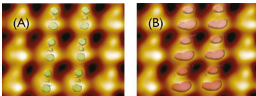
Figure 19. STM image of (\text{EDO-TTF})_2\text{PF}_6 with (A) the simulated constant charge density contour of 3 \times 10^{-8} \text{ nm}^{-3} at 2 \text{ \AA} from the oxygen atom. The second oxygen and the second carbon contribute only a little. The small spots are assigned to the second half of \text{O}_{2p} orbital and with (B) the simulation by the rotational reconstruction model with the condition of \theta_a = 18^\circ , \theta_b = 29^\circ as described in Figure 20 , which successfully reproduces the overall profile of the observed image.
