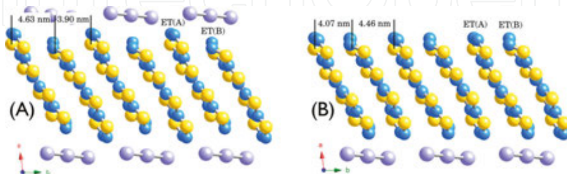
Figure 13. (A) Crystal structure of \beta -(ET) 2 I 3 projected along the c axis with three unit cells. ET(A) is located nearer to the b - c surface by \approx 0.1 nm than ET(B). (B) A model for the surface layer of \beta -(ET) 2 I 3 . ET(B)s are slid to align TTF double bonds to the same height as that of ET(A), which increases the cohesive energy in the surface ET layer. The separations between ET(A) and ET(B) are contrasted to (A). The topmost sulfur atoms of ET(B) are slightly deeper by 0.01 nm than ET(A).
