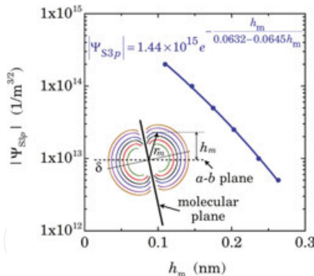
Figure 5. Maximum height h_m estimated from each \Psi_{S3p} wavefunction contour in the inset, where the symmetry axis (thin solid line) of the 3p wavefunction tilts by \delta \approx 12 deg against the a - b plane described by the dashed horizontal line through the sulfur atom. The analytical expression approximately describes |\Psi_{S3p}| as a function of h_m , which is applicable to the STM topography analysis in the a - b plane of \alpha -(ET) _2 I _3 (reused from Ref. [1]).
