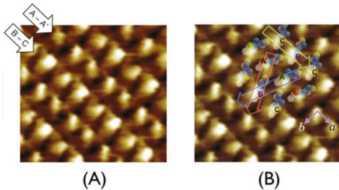
Figure 9. STM image of \alpha -(BEDT-TTF) 2 I 3 in 2.8 \times 2.6 nm 2 . Four BEDT-TTF molecules are contained in the unit cell. (A) Molecular arrays, A–A' and B–C, run from the top left to the right bottom. (B) Crystal structure assigned to the STM image of \alpha -(BEDT-TTF) 2 I 3 . The balls with A', A, B, and C represent the relevant sulfur atoms. The three large arrows represent the direction of the topography shown in Figure 10 (reused from Ref. [1]).
