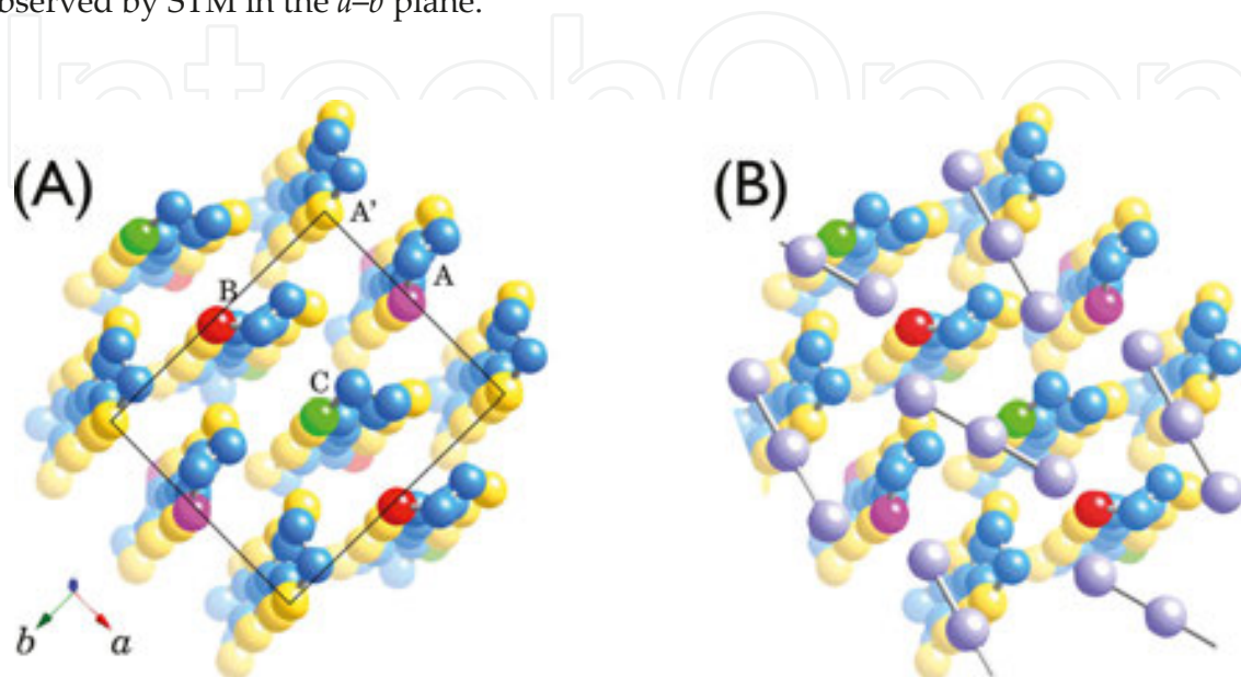
Figure 6. Unit cell structure of \alpha -(ET) 2 I 3 determined by the X-ray analysis at 300 K [23]. Blue and yellow balls indicate carbon and sulfur atoms, respectively. Hydrogen atoms are not indicated. The labels A, A', B, and C show the four molecules in a unit cell. The sulfur atoms observed by STM are marked by the special colors of purple, yellow, red and green for A, A', B, and C molecules, respectively. a = 0.9187 nm, b = 1.0793 nm, c = 1.7400 nm, \alpha = 96.957^\circ , \beta = 97.911^\circ , and \gamma = 90.795^\circ . (B) shows relative location of I 3 - ions.
