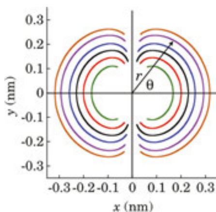
Figure 4. Constant amplitude contour of 3p wavefunction of a sulfur atom deduced from Figure 3 for the STM topography analysis in \alpha -(ET) 2 I 3 . The abscissa corresponds to the symmetry axis of the 3p orbital of the sulfur atom at the origin, perpendicular to the molecular plane corresponding to the vertical line. Each constant amplitude of |\Psi_{S3p}| is 5 \times 10^{12}, 1 \times 10^{13}, 5 \times 10^{13}, 1 \times 10^{14}, and 2 \times 10^{14} m^{-3/2} from the outer to the inner (reused from Ref. [1]).
