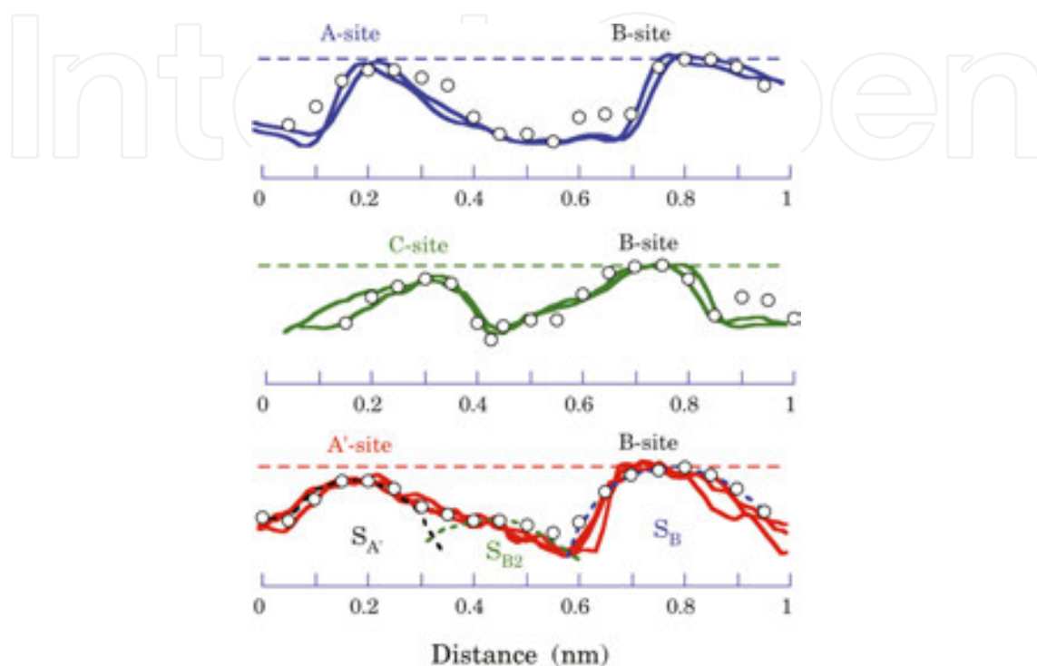
Figure 10. STM topographies of \alpha -(BEDT-TTF) _2 I _3 (solid curves) and the simulations (open circles) with \sum_i |\Psi_{S3p}^i|^2 , where the molecular charge ratio \rho_i / \rho_B in Table 1 was taken into account. The topographies were measured along the arrows in Figure 9(B) . The horizontal dashed straight lines are visual guides at the top of the S_B site. The broken curves for the bottom A–B scan show individual contributions of each sulfur atom at S_B and S_{A'} and S_{B2} . From S_{B'} , note that S_{B2} is 0.1 nm inside. The vertical scale is the same as the horizontal one (reused from Ref. [1]).
