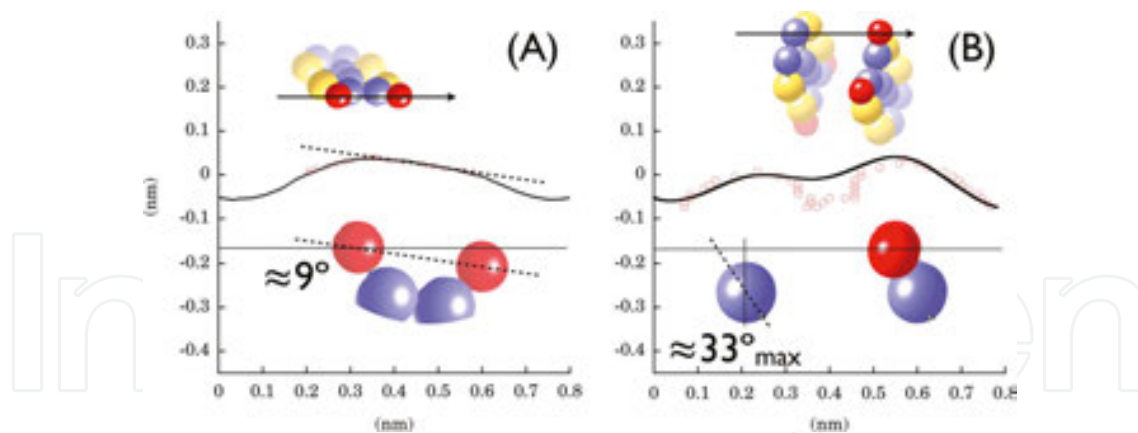
Figure 21. The topographies (A) along the oxygen pair of EDO group and (B) along the oxygen and the carbon atoms of the EDO-TTF molecules. The circles represent the simulated profile at the \pi charge density of 1 \times 10^{-5} \text{ nm}^{-3} with \theta_a = 18^\circ , \theta_b = 29^\circ . The horizontal line indicates the relative position of the oxygen atom.
