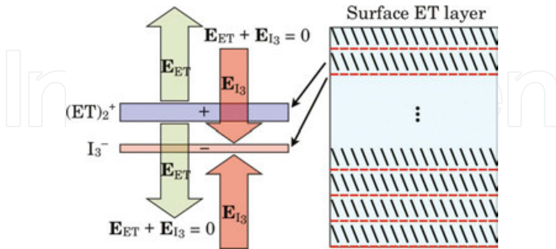
Figure 1. Schematic picture of the electric field produced by a (\text{ET})_2^+ and \text{I}_3^- double layer with the same total charges of each layer in \alpha\text{-(BEDT-TTF)}_2\text{I}_3 . The electric field of the double layer is confined inside the double layer. That is, outside the double layer, the electric field cancels out. However, the leakage electric field near the double layer forms the electric dipolar field, which binds the neighboring double layers. Thus, the surface ET layer approximately feels only the electric field of the \text{I}_3^- layer within the double layer (reused from Ref. [1]).
