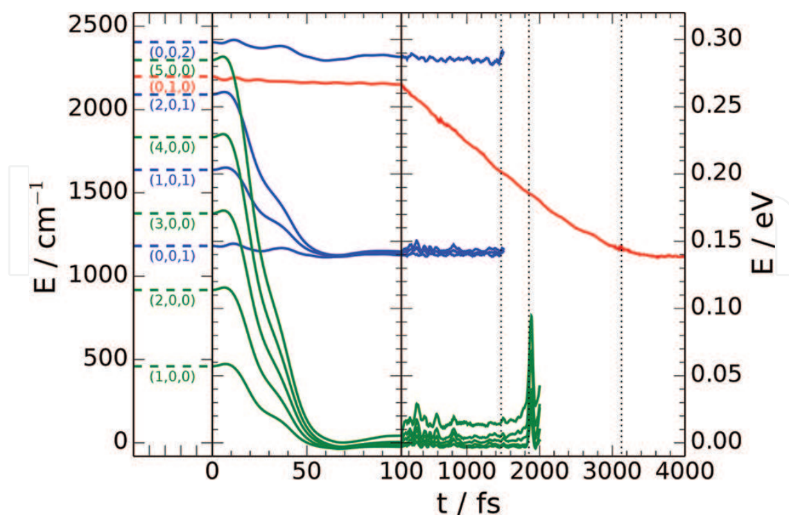
Figure 6. Time evolution of the system energy for the lowest lying vibrational states of the CH potential, computed with MCTDH and here labeled by the three appropriate quantum numbers (v_{s,CH}, v_{s,surf}, v_b) where v_{s,CH} is the C–H stretching, v_{s,surf} is the surface stretching, and v_b is the doubly degenerate C–H bending. The panel on the left gives the vibrational energy spectrum of the system. The dashed lines mark the recurrence time of the bath models adopted.
