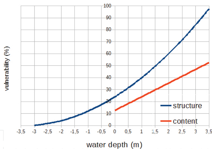
Figure 9. Vulnerability curve adopted in the implemented model.
