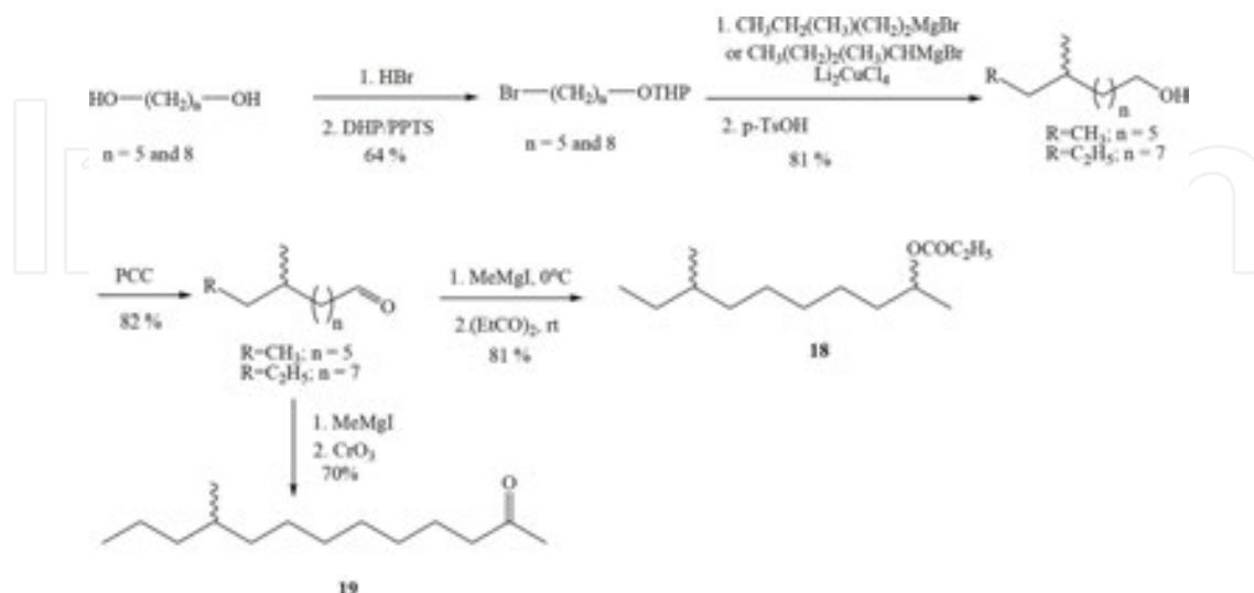
Scheme 7. Synthetic route of 8-methyldec-2-yl propanoate and 10-methyl-2-tridecanone.
