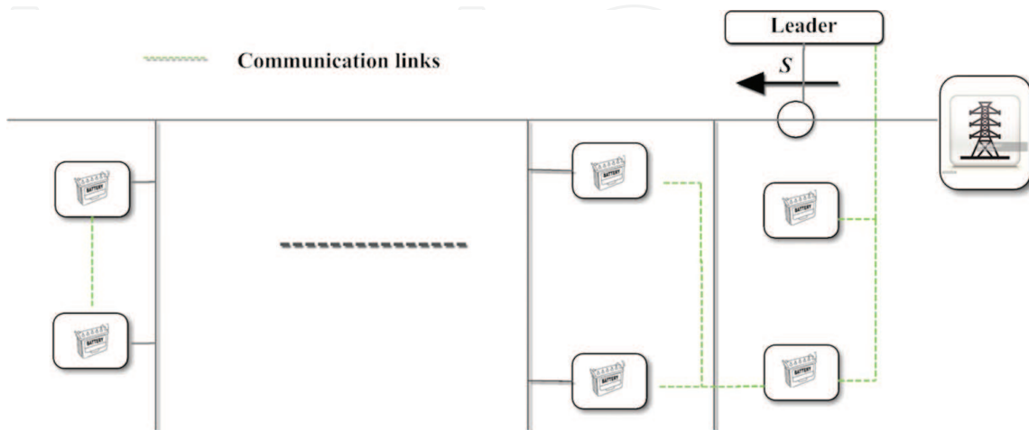
Figure 2. Distributed control structure for distribution network.
