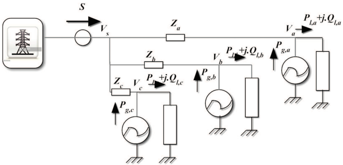
Figure 1. Distribution network equivalent, with renewable energy sources.
