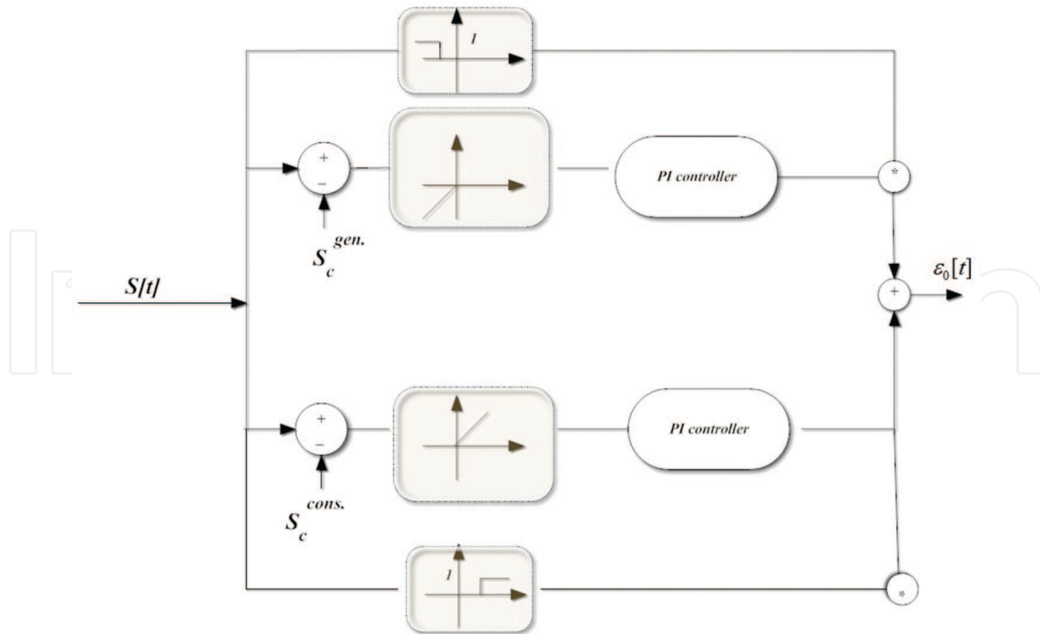
Figure 4. Leader control structure for ESS fair contribution.
