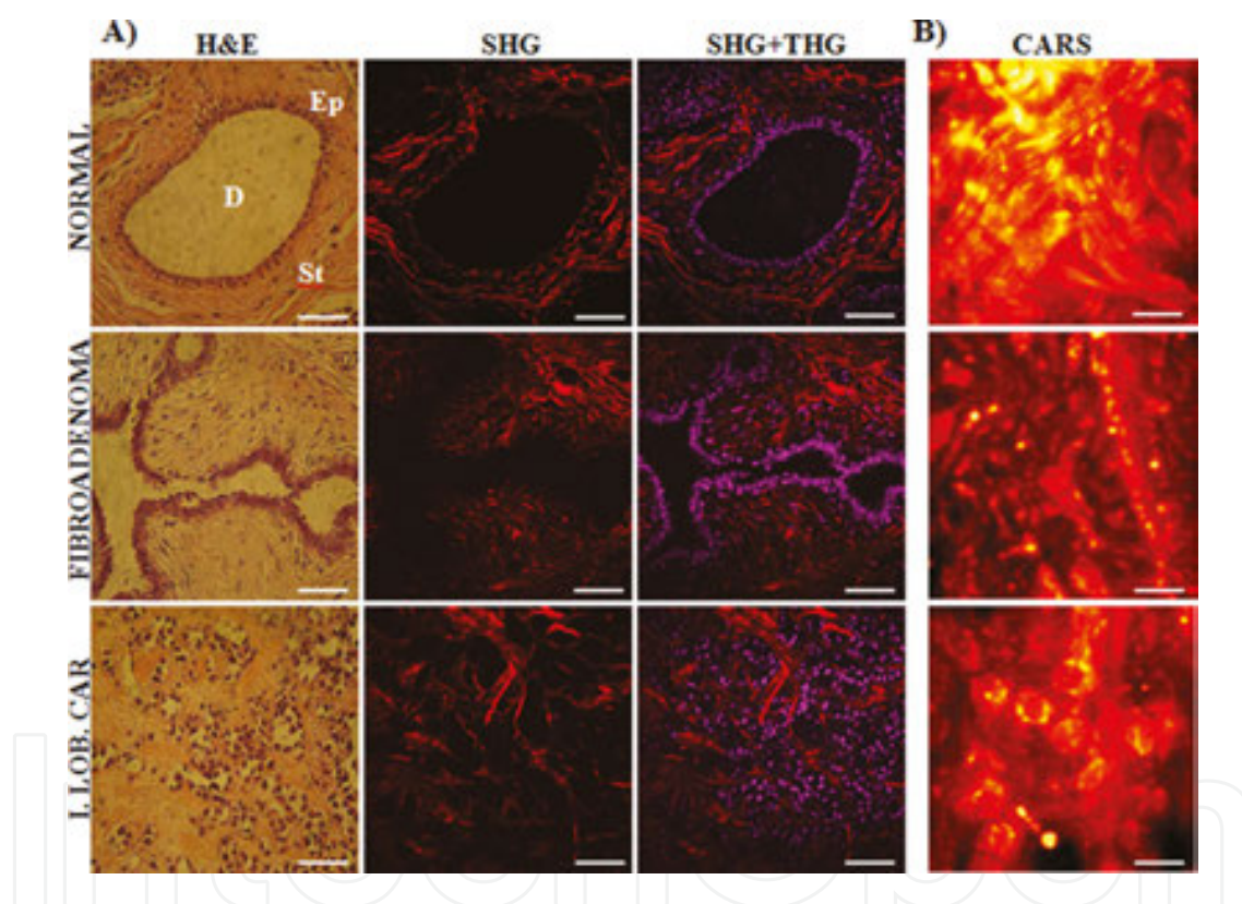
Figure 3. Multimodal NLO approach applied to human breast tumor. (A) Representative H&E-stained and SHG, and SHG+THG cross-sectional images of breast tissues diagnosed as normal (first row), fibroadenoma (second row), and invasive lobular carcinoma (third row). Scale bar = 20 \mu m. (B) Representative CARS cross-sectional images of breast tissues. Scale bar = 20 \mu m. D, duct; Ep, epithelium; St, stroma; Fibroad, fibroadenoma; Lob. Carc., lobular carcinoma; I.Lob.Carc, invasive lobular carcinoma. Figure 3A from Adur et al., [19].
