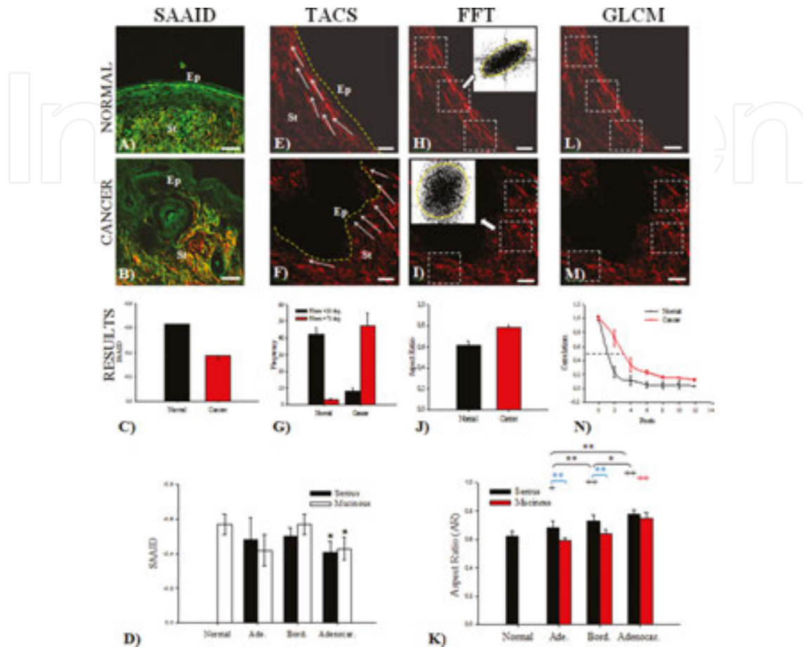
Figure 7. Depicting several applications of different methods to analyze NLO signals. The panel shows representative TPEF (green) and SHG (red) images of (A, E, H, L) normal and (B, F, I, M) cancer ovary. From the TPEF+SHG combination (first column), it is possible to calculate (C) the SAAID ratio. From the SHG image (remaining columns) and using regions near the epithelial/stromal interface (yellow line), it is possible to calculate: (G) TACS (measuring the collagen fiber angle relative to the epithelium); (J) FFT transforms (and fit to ellipse to estimate the anisotropy); and (N) GLCM (correlation value). (D) Bar graphs represent SAAID index quantitative analysis of ovarian tissues. Asterisks indicate a significant increase as compared to the nontumor tissues ( p < 0.05 , t -test). (K) Bar graphs represent anisotropy (aspect ratio) quantitative analysis of ovarian tissues. Comparisons with normal tissues are indicated with +, +,* indicates a statistically significant ( p < 0.05 ) difference and ++, ** indicates a statistically very significant ( p < 0.01 ) difference following ANOVA. Ep, epithelium; St, stroma; white arrows, collagen fibers; white squares, regions of interest (ROI). Reproduced figures from Adur et al. [4] (open access).
