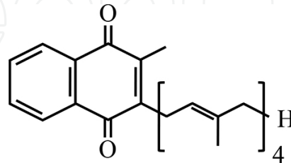
Figure 1. Chemical structure of MK-4. MK-4 has a 2-methyl-1,4-naphthoquinone ring and a geranylgeranyl group (four isoprene units) as a side chain.
