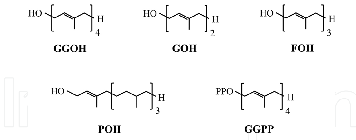
Figure 6. Chemical structures of isoprenoid groups; geranylgeraniol (GGOH), geraniol (GOH), farnesol (FOH), phytol (POH), and geranylgeranyl diphosphate (GGPP).
