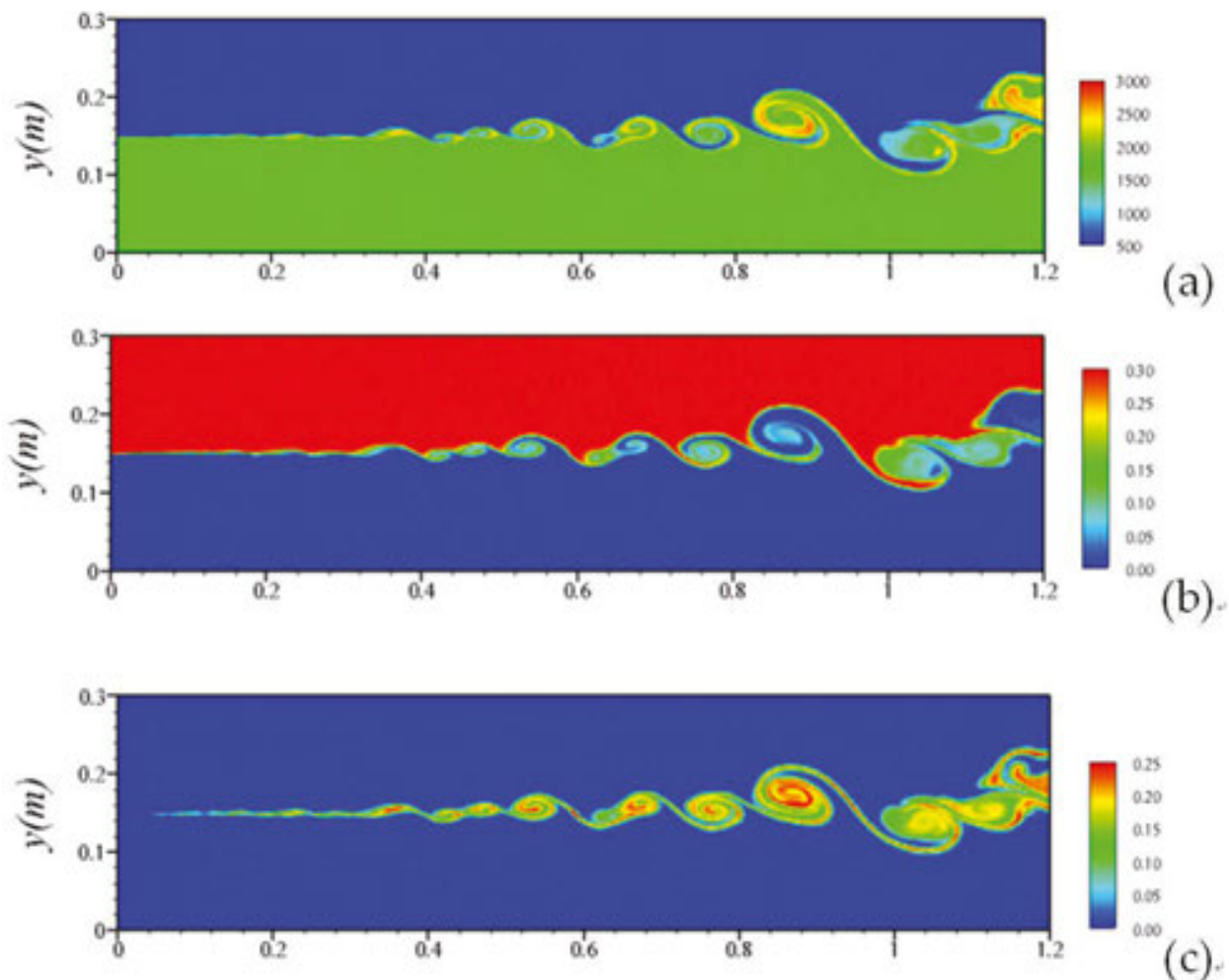
Figure 7. Instantaneous contour distribution of reactive flows. (a) temperature; (b) H_2 ; (c) H_2O .
