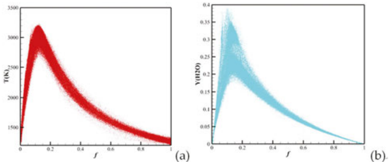
Figure 8. Flame structure. (a) temperature distribution and (b) water distribution.
