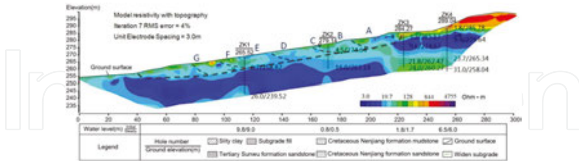
Figure 10. Comparison of drilling results and electrical resistivity profile of the survey line I-I'. Geological drilling date is in June 2010, HDR detection date is on September 3, 2012. The dashed thick black line indicates the position of the major sliding surface, and the dashed thin black lines illustrate the secondary sliding surfaces.
