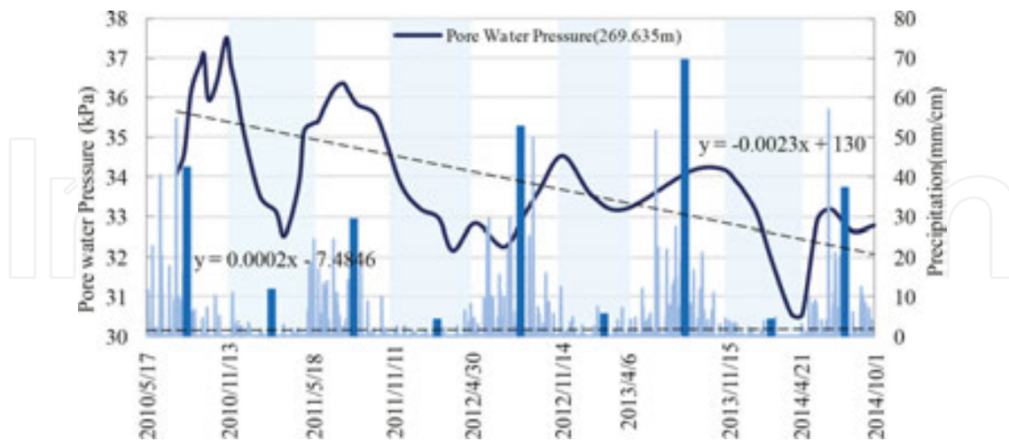
Figure 26. Daily precipitation and pore water pressure in the depth of 19.4 cm of ZK4 point in K178 + 530 section of Bei'an-Heihe Highway.
