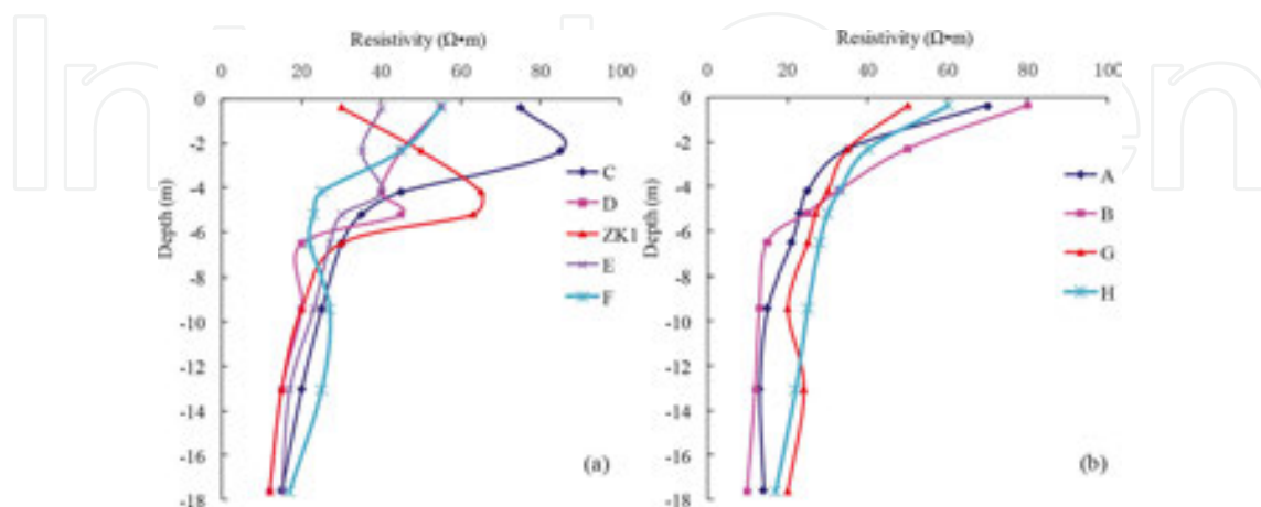
Figure 14. The electrical resistivity curves at different points on the survey line II-II' (points C, D, ZK1, E and F are all on the landslide mass, points A, B, G and H are all outside the landslide mass).
