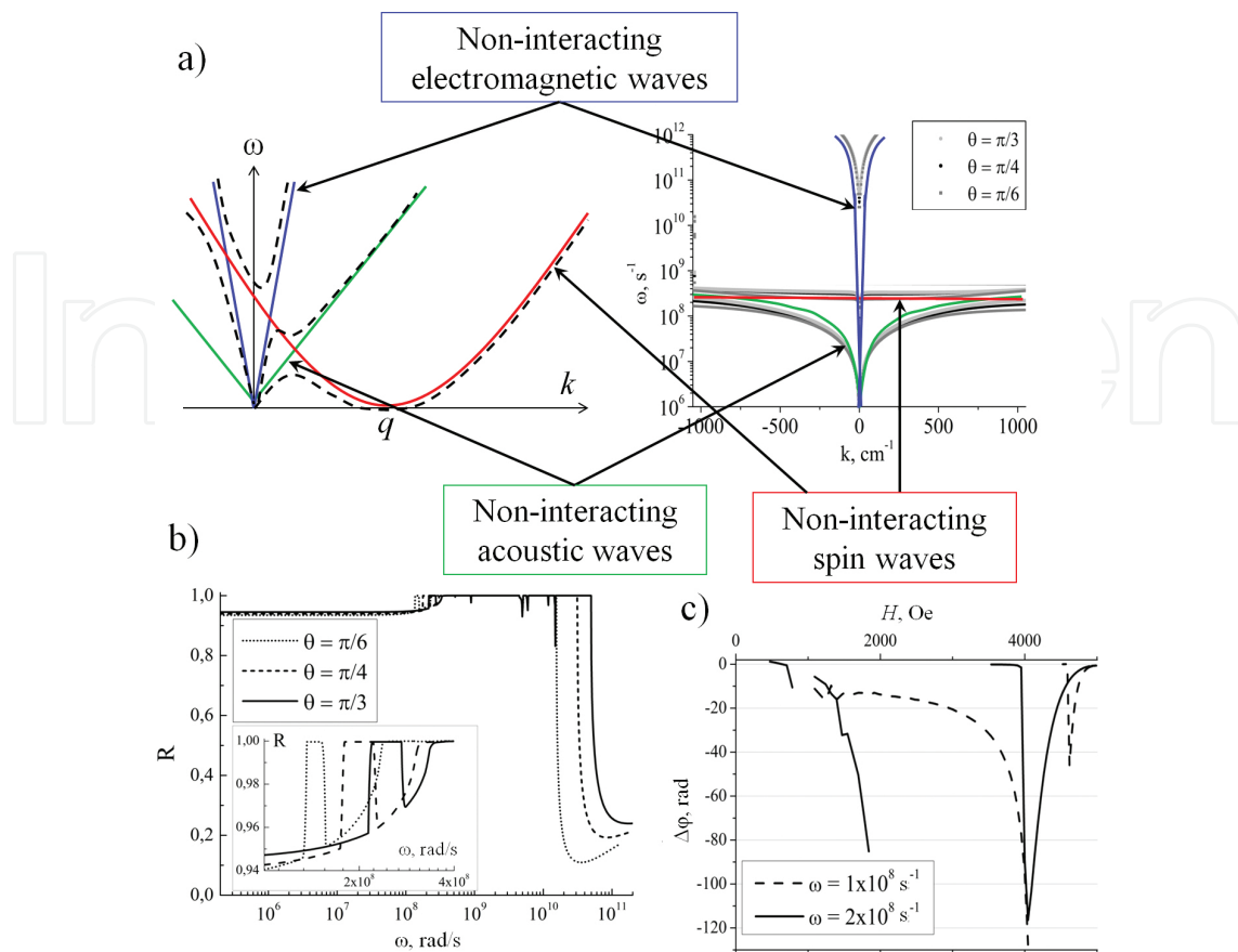
Figure 2. Spectrum of coupled waves (a) (left – schematic spectrum, right – calculated spectrum near k = 0 ). Electromagnetic waves reflection from semi-infinite spiral magnet (b). On the inset the feature associated with the acoustic gap is shown. Acoustic Faraday effect (c).
