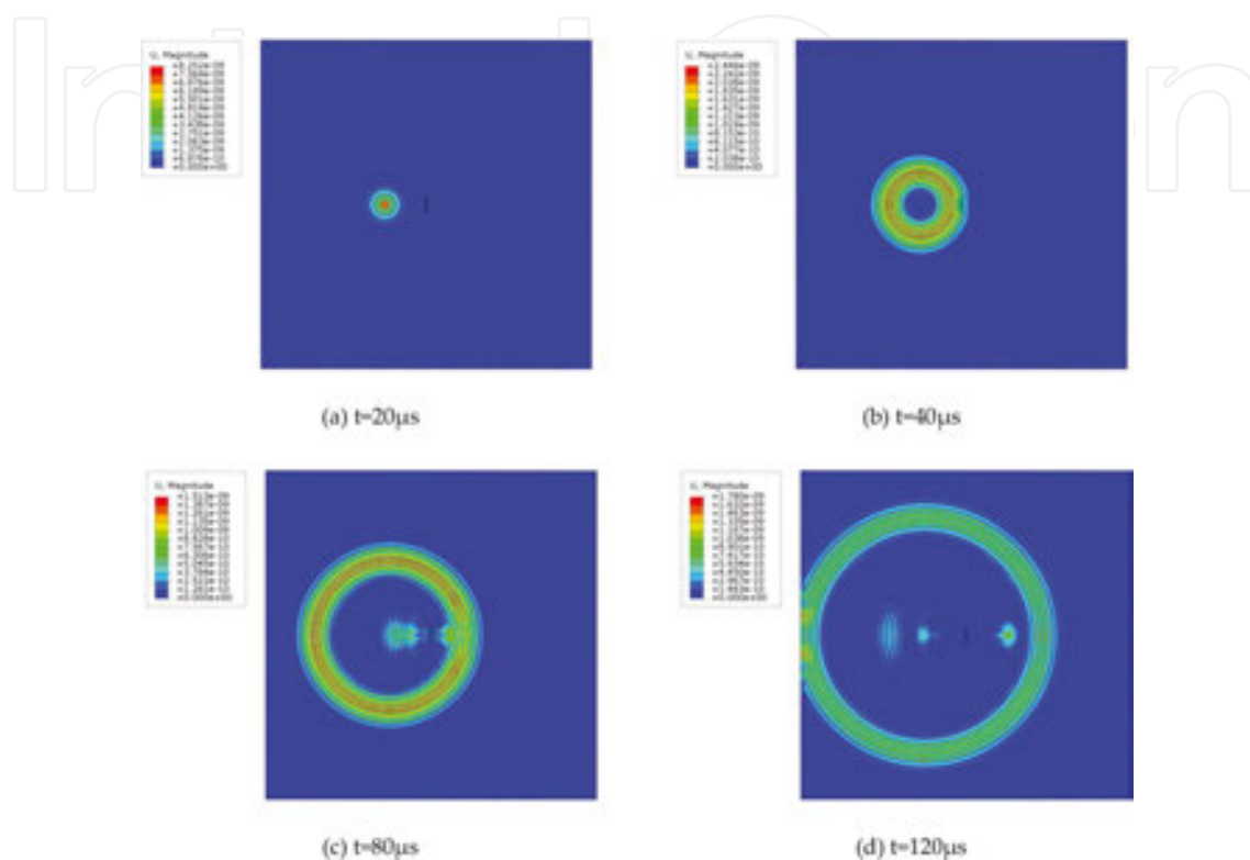
Figure 9. The scattering field of a through-thickness crack.
