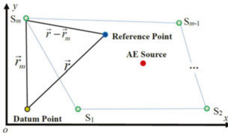
Figure 10. Principle illustration of the beamforming network method.
