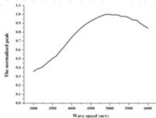
Figure 19. The normalized energy peak curves of 8 mm steel cylinder with different wave speeds.
