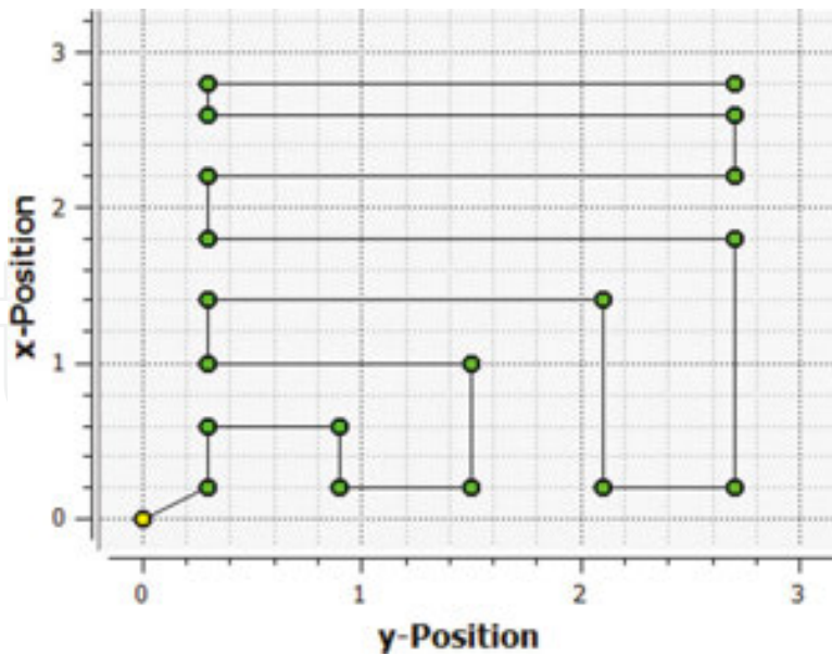
Figure 2. BFS waypoint list (VFOV 40 \times 60 ).
