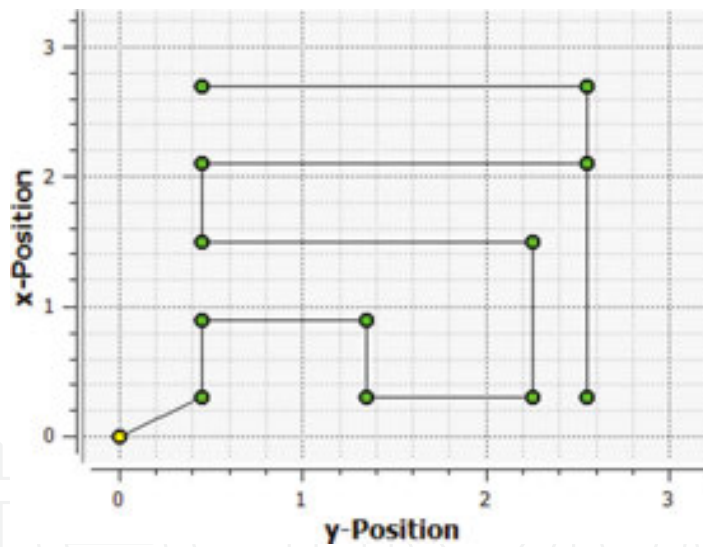
Figure 3. BFS waypoint list (VFOV 60 \times 90 ).
