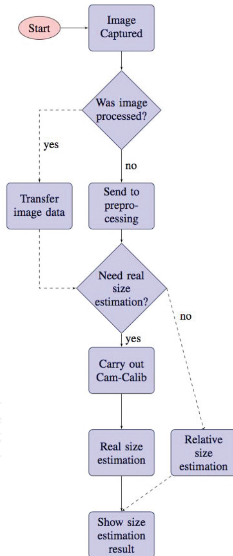
Figure 10. Size estimation with segmentation flowchart.
