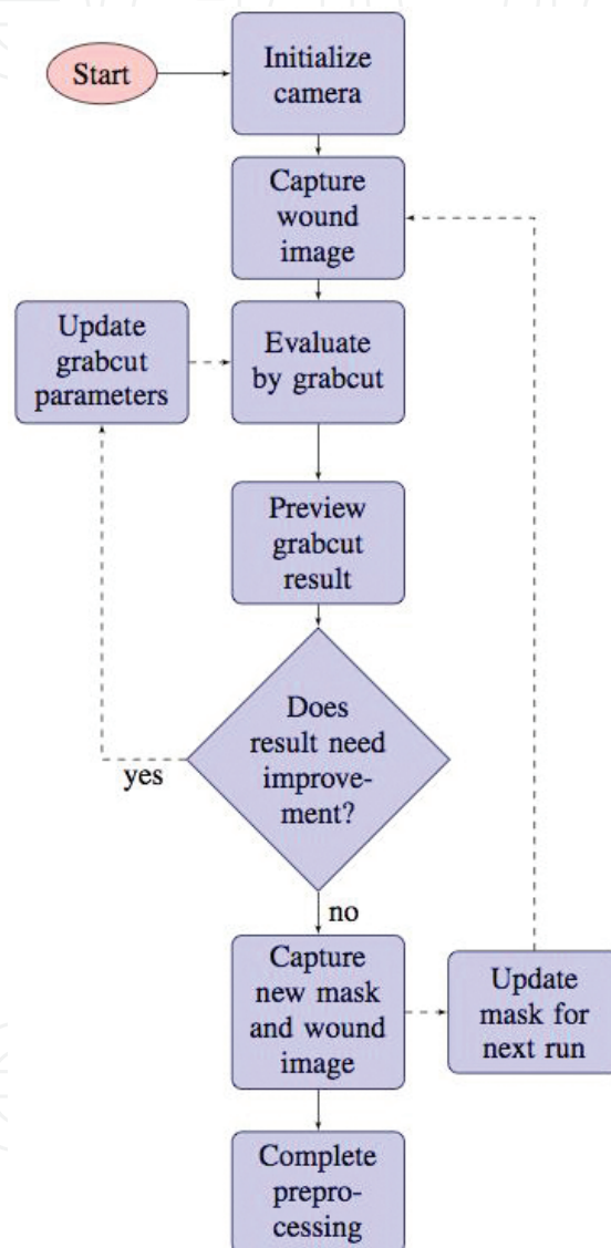
Figure 7. Image acquisition and pre-processing flowchart.
