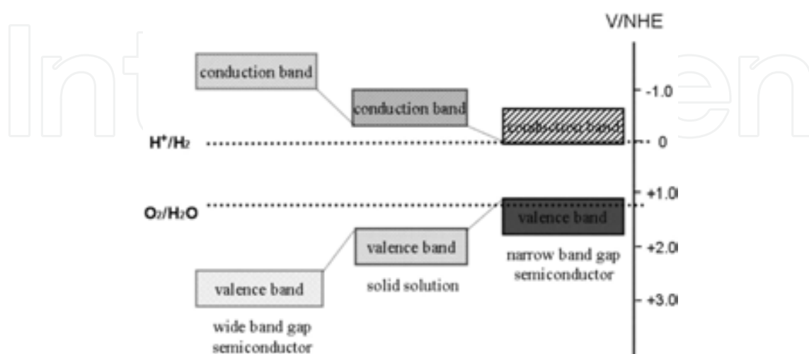
Figure 6. Band structure controlled by making a solid solution [11].
