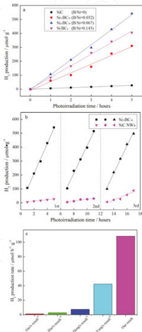
Figure 18. (a). Photocatalytic hydrogen evolution performance over B x SiC. (b). Hydrogen production rates of as-prepared the 3C-SiC NWs and B-doped 3C-SiC NWs. (c). The comparison of Hydrogen production rates.
