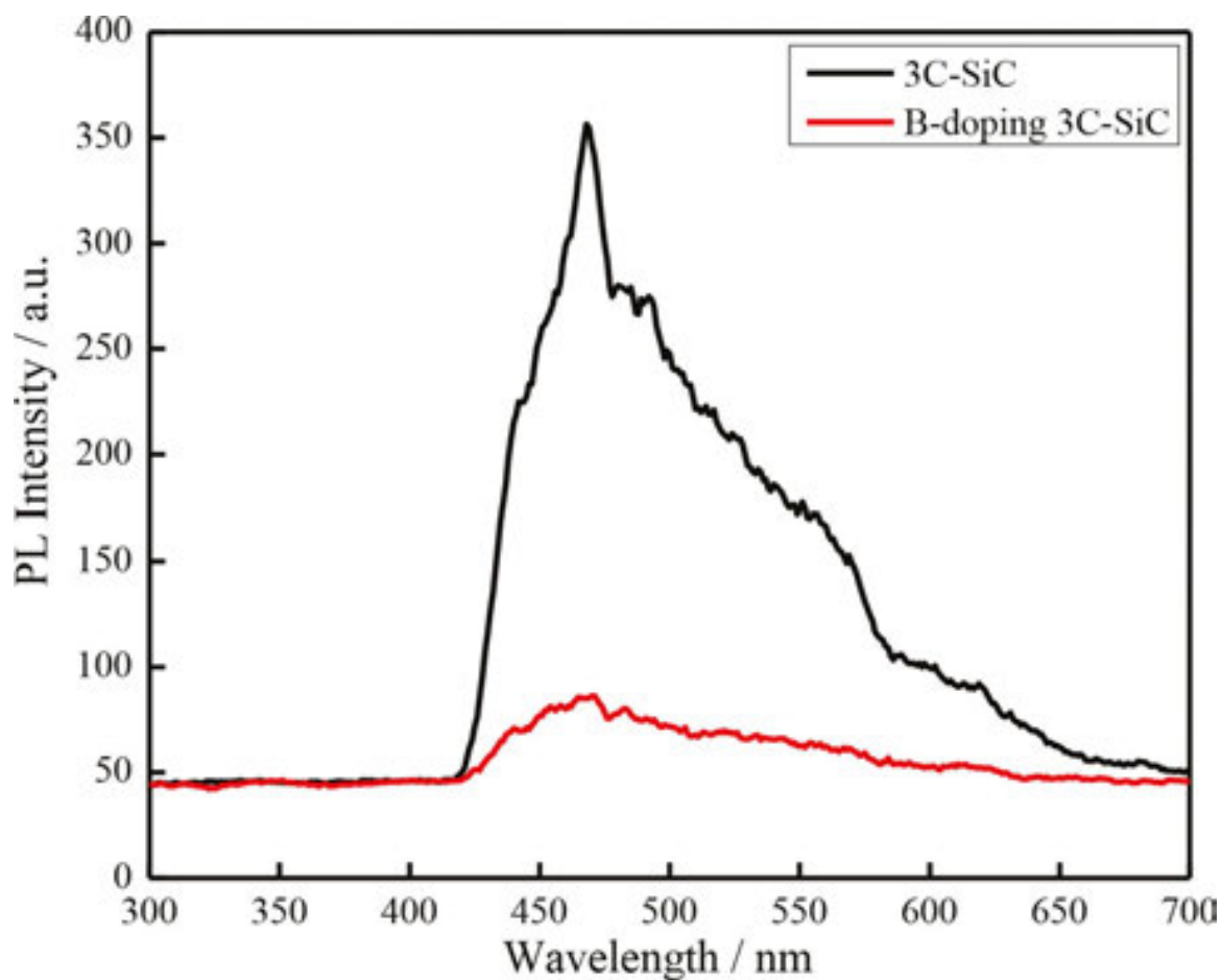
Figure 21. Photoluminescence spectra of 3C-SiC and B-doped 3C-SiC.
