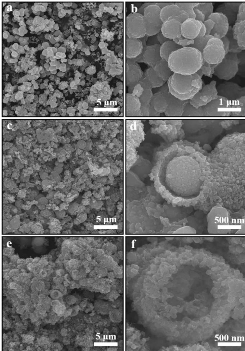
Figure 25. SEM photographs of TiO x N y /TiN composites: (a), (b) solid, (c), (d) yolk-shell, (e), (f) hollow.
