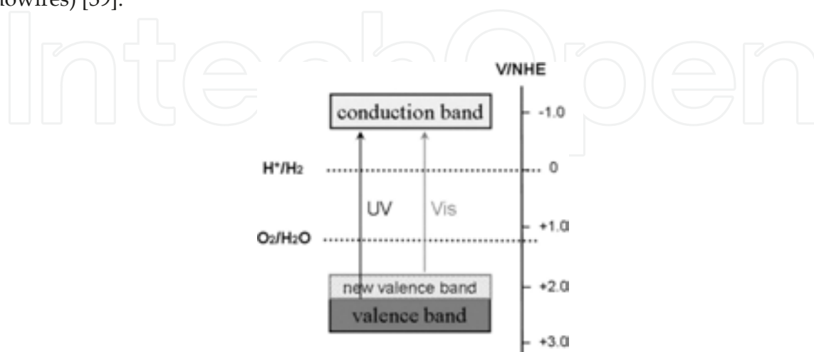
Figure 5. New valence band formation by doping of nonmetal ions [11].
