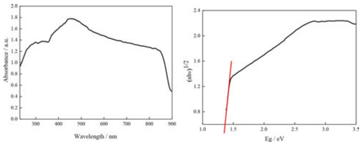
Figure 28. (a) UV-Vis diffuse reflection spectra of yolk-shell \text{TiO}_x\text{N}_y/\text{TiN} . (b) The plots of (ah\nu)^{1/2} versus h\nu . The band gap of yolk-shell \text{TiO}_x\text{N}_y/\text{TiN} .
