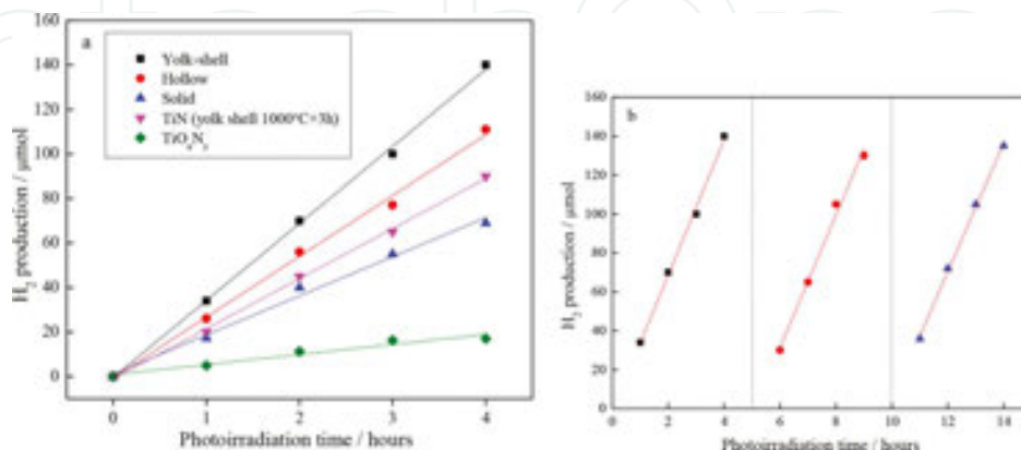
Figure 27. (a). Comparison of \text{H}_2 production rates of \text{TiN} , \text{TiO}_x\text{N}_y and \text{TiO}_x\text{N}_y/\text{TiN} heterojunction with different nanostructure. (b). Recycling test of the yolk-shell \text{TiO}_x\text{N}_y/\text{TiN} in the photocatalytic \text{H}_2 evolution.
