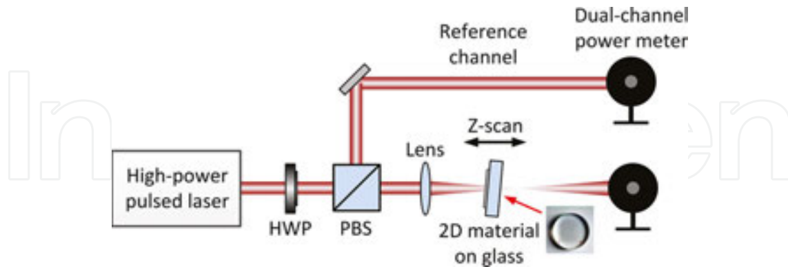
Figure 6. Power-dependent transmission measurement of a saturable absorber in free-space configuration.
