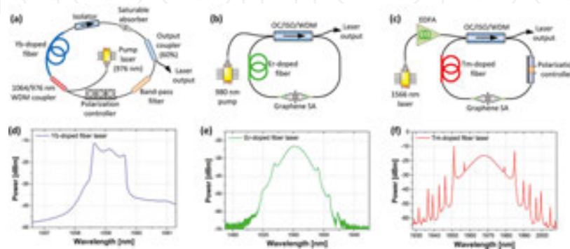
Figure 13. Fiber lasers operating at 1 \mu\text{m} (a), 1.55 \mu\text{m} (b), and 1.97 \mu\text{m} (c), and the corresponding optical spectra generated by those lasers (d, e, f).
