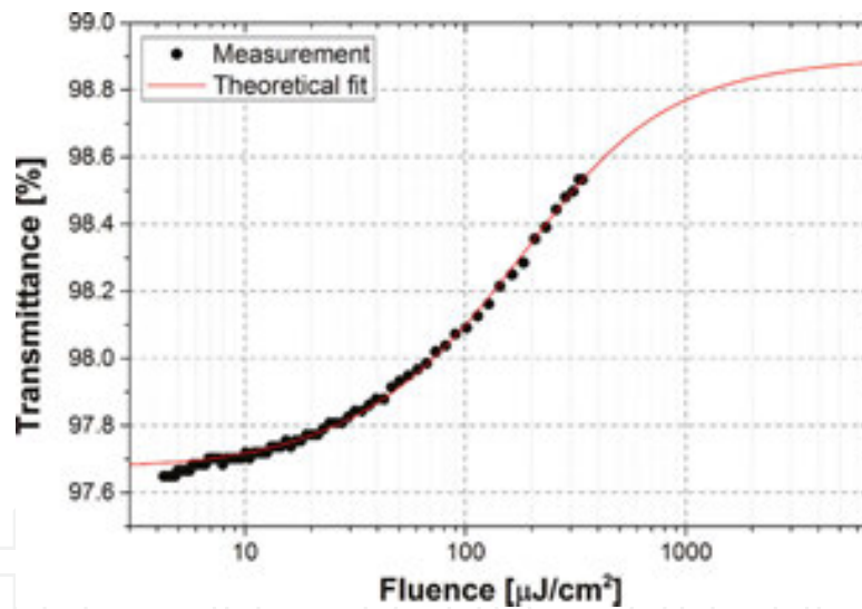
Figure 9. Measurement of saturable absorption in monolayer graphene.
