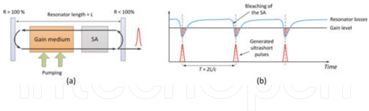
Figure 2. Illustration of a laser cavity with inserted saturable absorber (a) and pulse train formed in the cavity as a result of resonator loss modulation (b).
