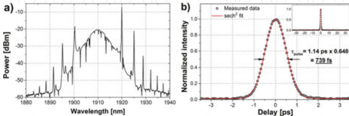
Figure 15. Optical spectrum generated by the BP mode-locked Tm-doped laser (a) and the autocorrelation trace of the emitted 739 fs pulse (b).
