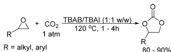
Scheme 1. Formation of cyclic carbonates in tetraalkylammonium salts.
