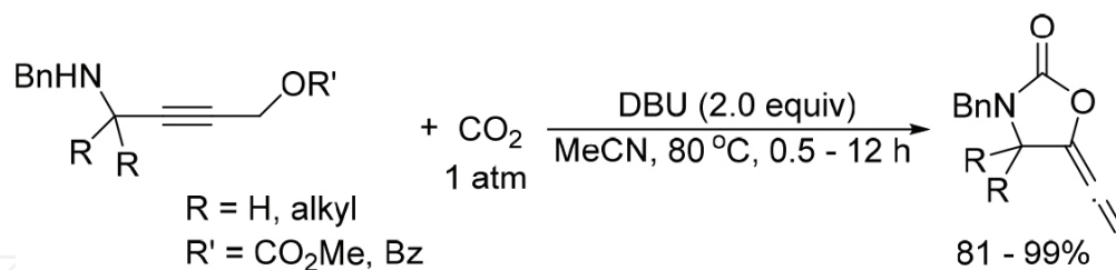
Scheme 15. DBU-mediated synthesis of substituted 5-vinylideneoxazolidin-2-ones.
