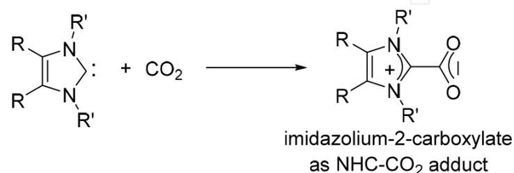
Scheme 22. Formation of NHC-CO 2 adduct.
