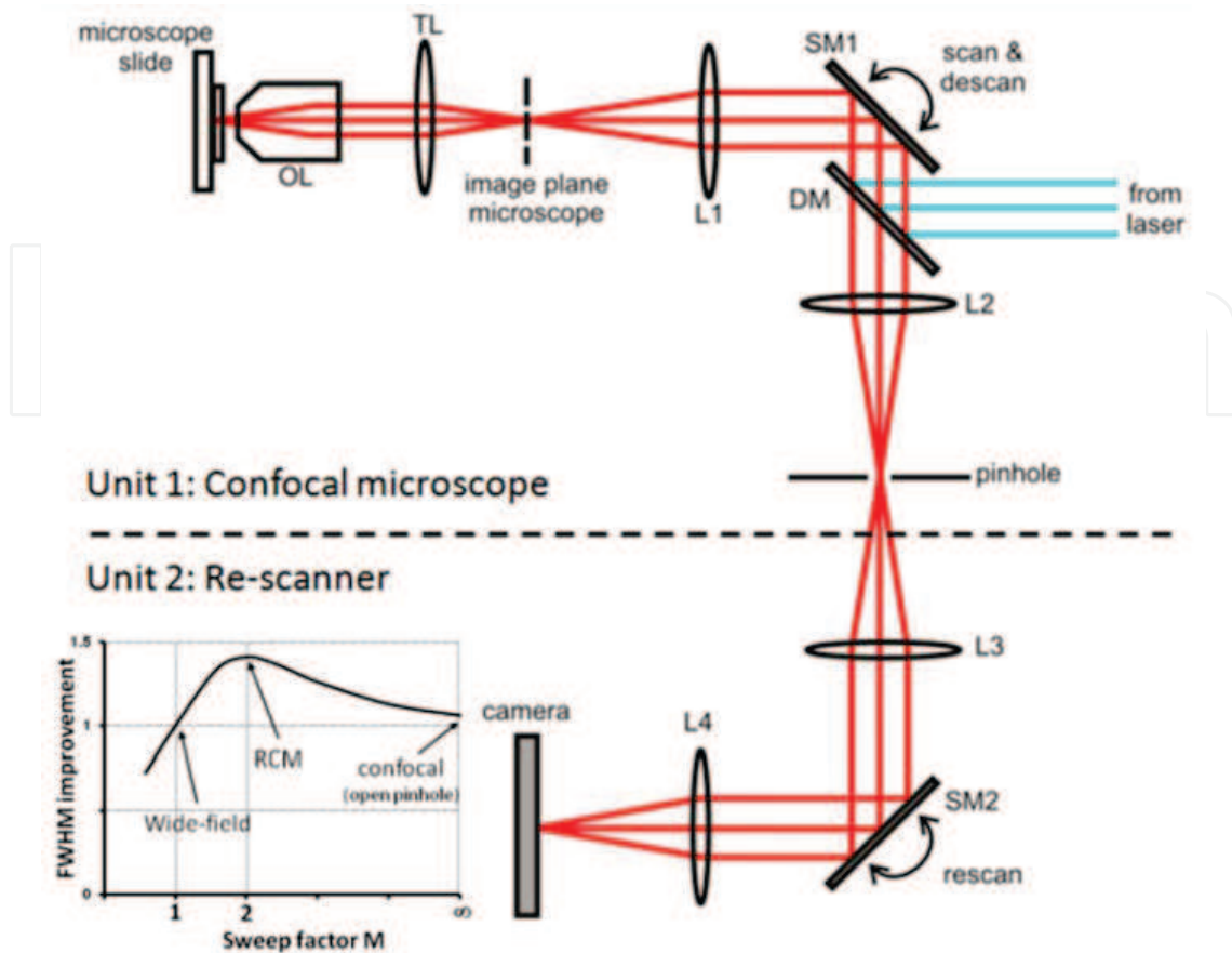
Figure 8. The schematic of rescan confocal microscopy (RCM). Unit 1: A standard confocal microscopy with a set of scanning mirrors for scanning the excitation light and de-scanning the emission light. Unit 2: A re-scanning configuration for ‘writing’ the light that passes the pinhole onto the CCD-camera. Although the pinhole is in a relatively large diameter, the resolution is \sqrt{2} times improved, which thus gives much more photo-efficient advantage compared to conventional confocal microscopes with the similar resolution. Adapted with permission from reference [12].
