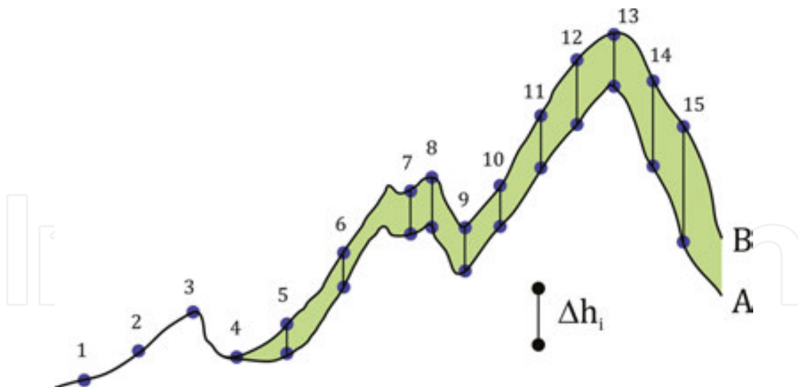
Figure 3. Schematic sketch of the DITs on the gravity change. Benchmarks 5 to 15, unlike 1 to 4, experienced a significant uplift ( \Delta h_i ). "A" denotes the predeformation topographic surface, whereas "B" denotes the postdeformation surface.
