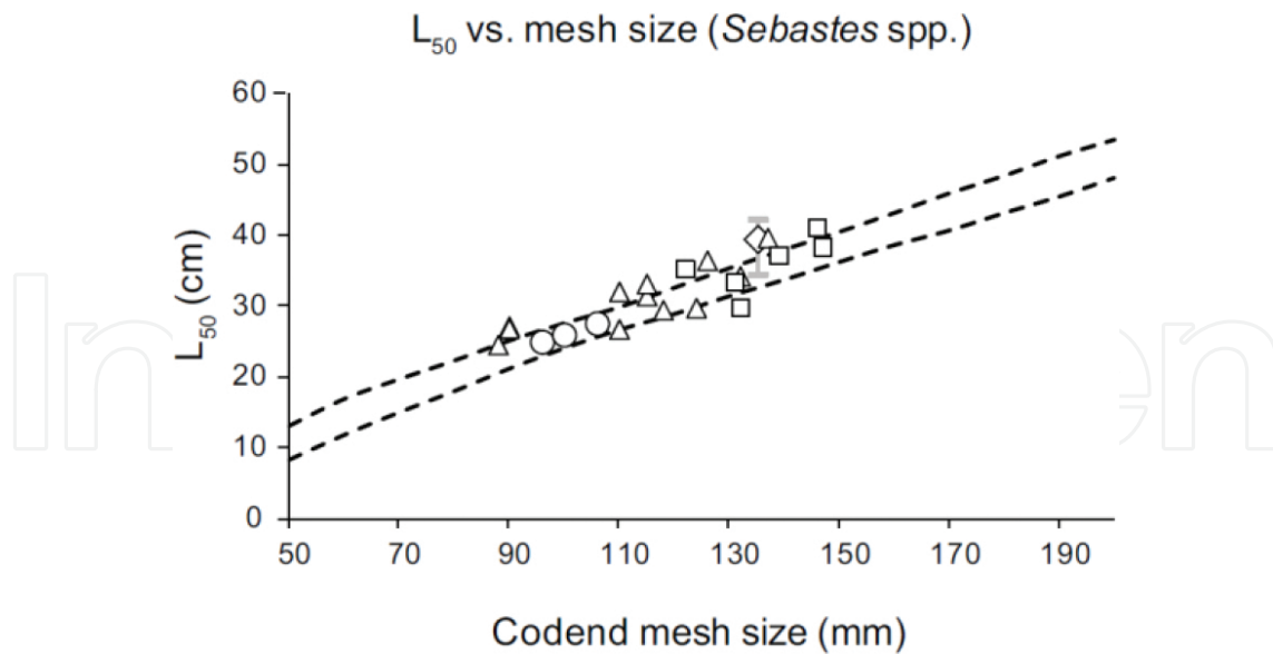
Figure 12. Predicted and observed L50 versus mesh size relationships for redfish ( Sebastes spp.): Predicted band for codend L50 for different mesh sizes based on the FISHSELECT analysis of the data collected for Sebastes marinus (stippled curves); new results from sea trials for S. marinus (diamonds); previous results for S. marinus (squares); previous results for Sebastes mentella (triangles) and Sebastes mentellafaciatus (circles). Source: [38].
