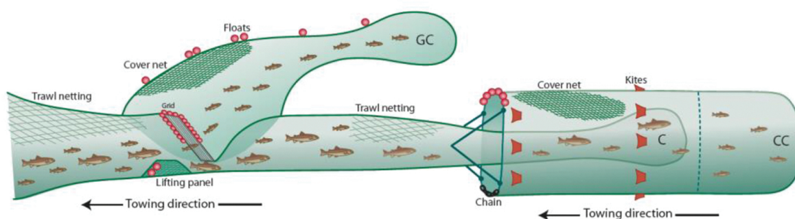
Figure 5. Dual cover method.
