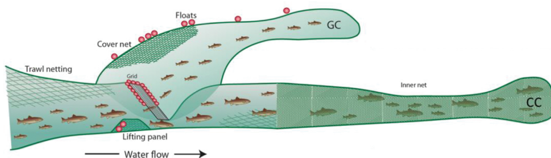
Figure 6. The Covered-grid method.
