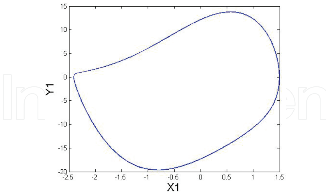
Figure 2. Phase portrait for reference model without feedback and delay, see first part of Eq. (5).
