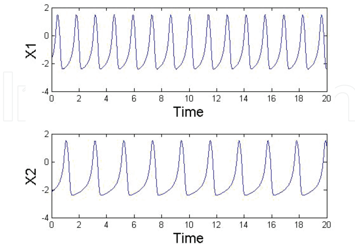
Figure 1. Time series for reference model without feedback and delay, see Eq. (5).
