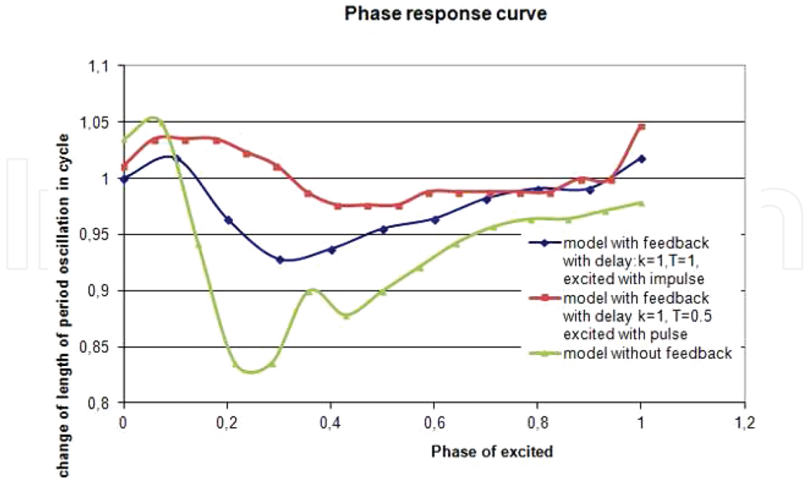
Figure 7. Phase response curves for models with rectangular pulse.
