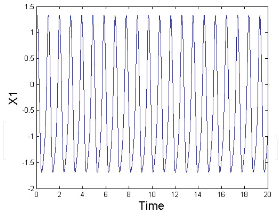
Figure 3. Dynamics of action potential during WPW syndrome.
