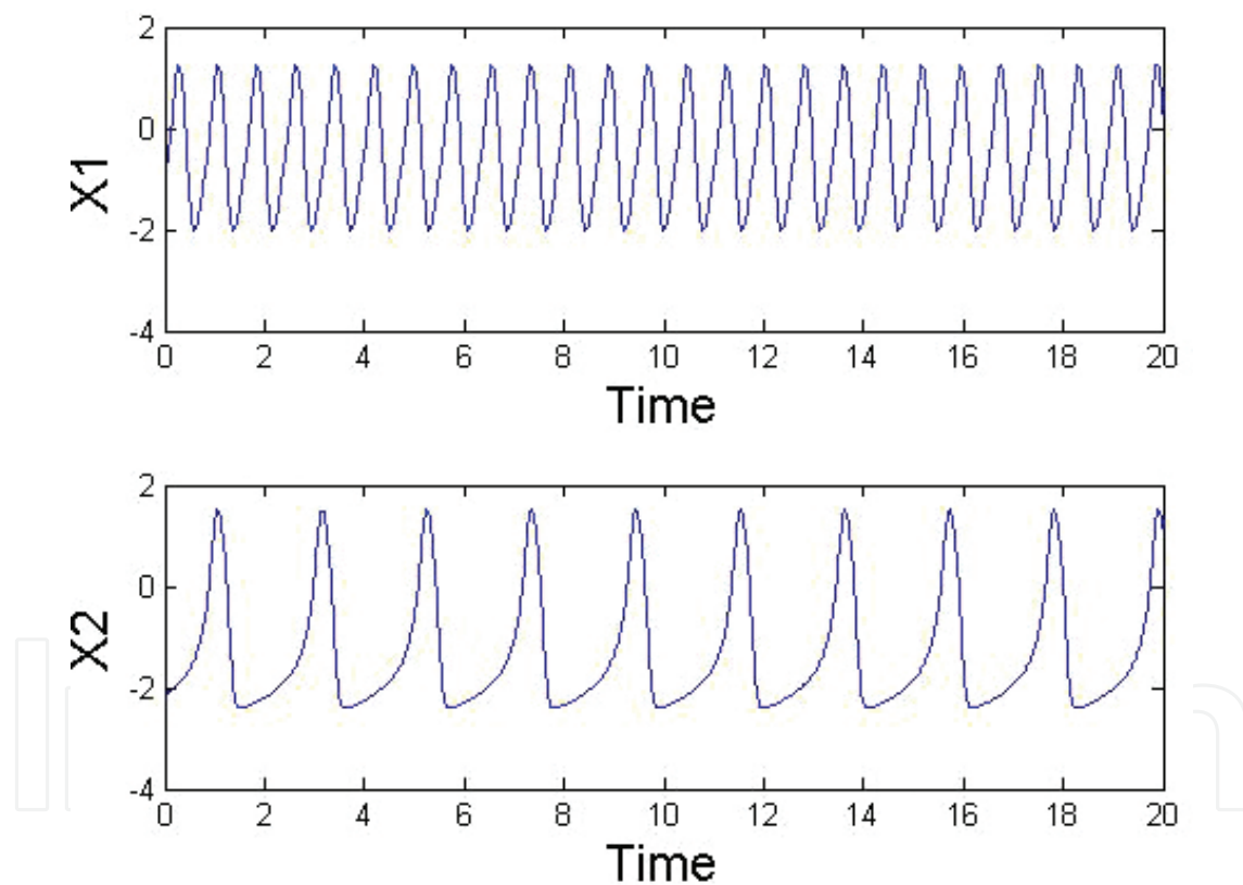
Figure 5. Dynamics of action potential for a typical AVNRT, given in Eq. (8).
