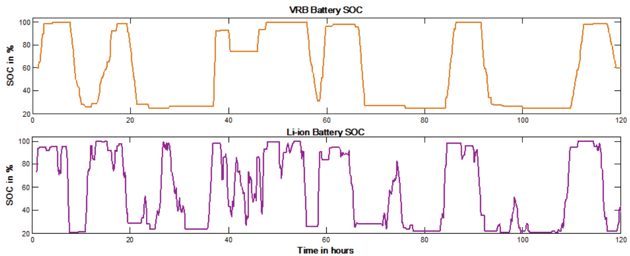
Figure 15. SOC of VRB and Li-ion battery.
