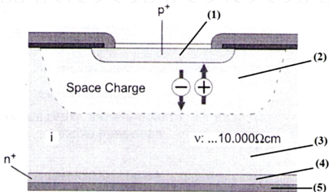
Figure 13. Cross-section of a PIN photodiode [41].
