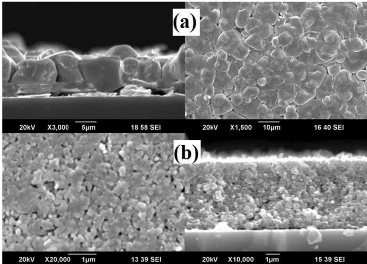
Figure 6. Morphology and cross-sections of oxide nanoparticles-based (a) CZTSe and (b) CZTS thin films [36, 37].
