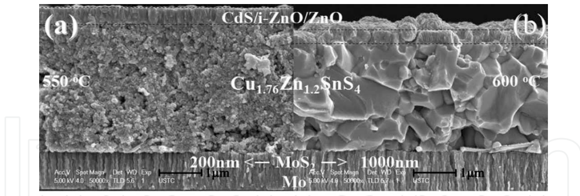
Figure 7. Cross-sectional SEM micrographs of photovoltaic devices using oxide nanoparticles-based CZTS thin films annealed under (a) 550°C and (b) 600°C [37].
