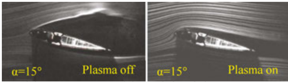
Figure 13. Flow structure around NACA0015 airfoil at Re = 15000 without (left-hand side) and with (right-hand side) plasma actuation [65].
