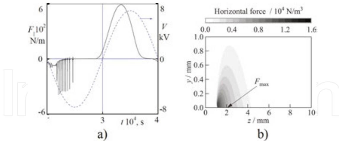
Figure 6. Time evolution of the EHD body force (a) [36], and spatial distribution of the average horizontal force (b) [33].
