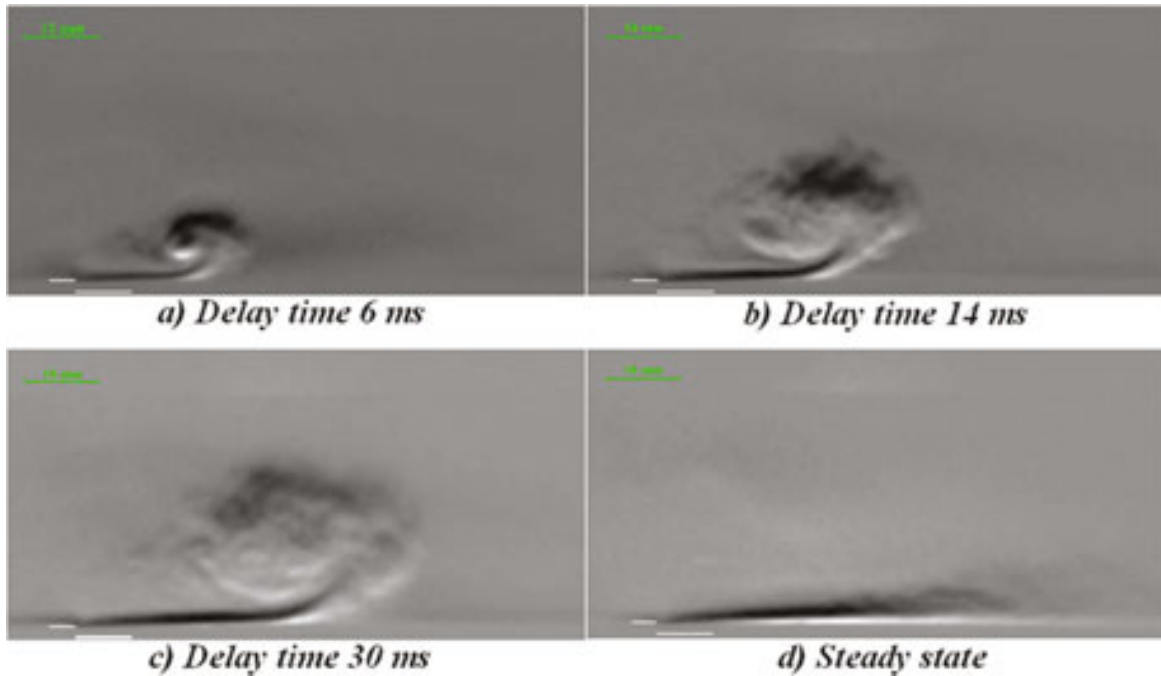
Figure 5. Schlieren images of induced wall jet during ignition phase of the discharge (a, b, and c) and steady state operation (d) [48].
