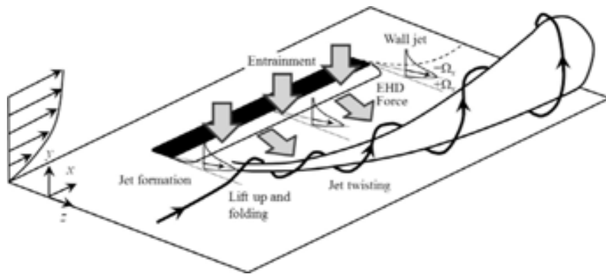
Figure 14. Vortex formation mechanism induced by a streamwise plasma actuator [8].
