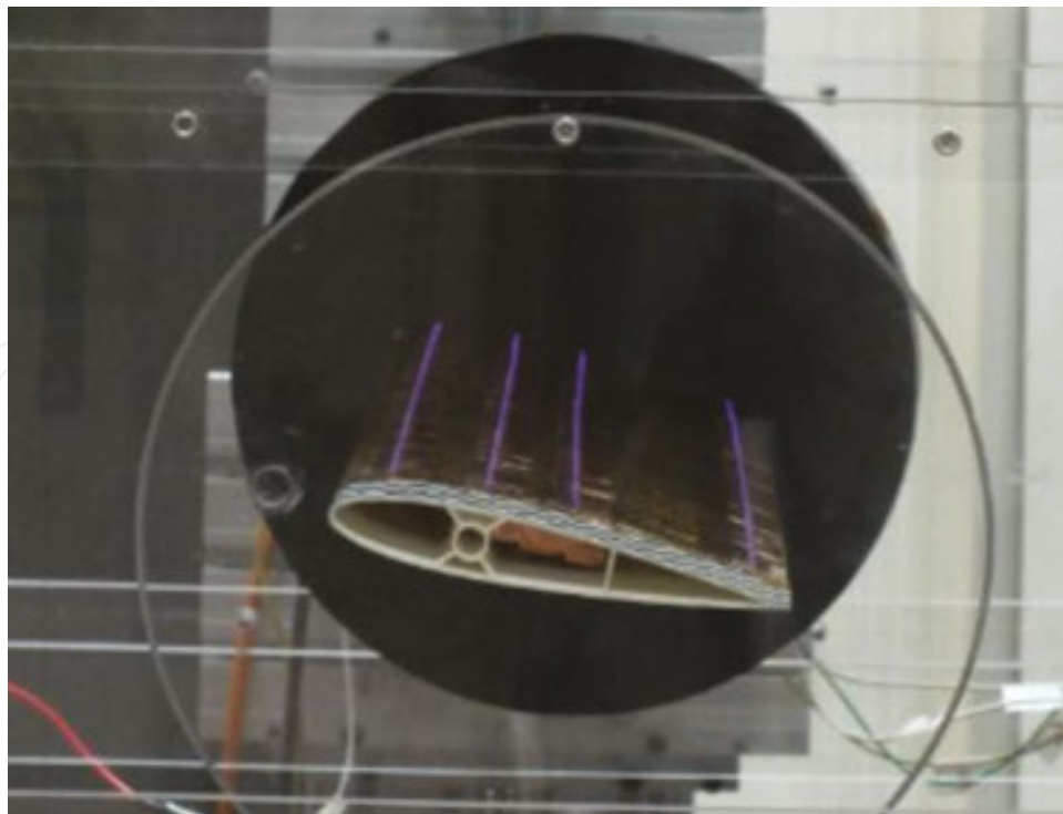
Figure 12. Airfoil equipped with four spanwise plasma actuators [65].
