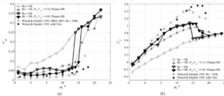
Figure 15. Drag (a) and lift coefficient enhancement (b) with counter-rotating PVGs on a NACA 4418 airfoil [8].
