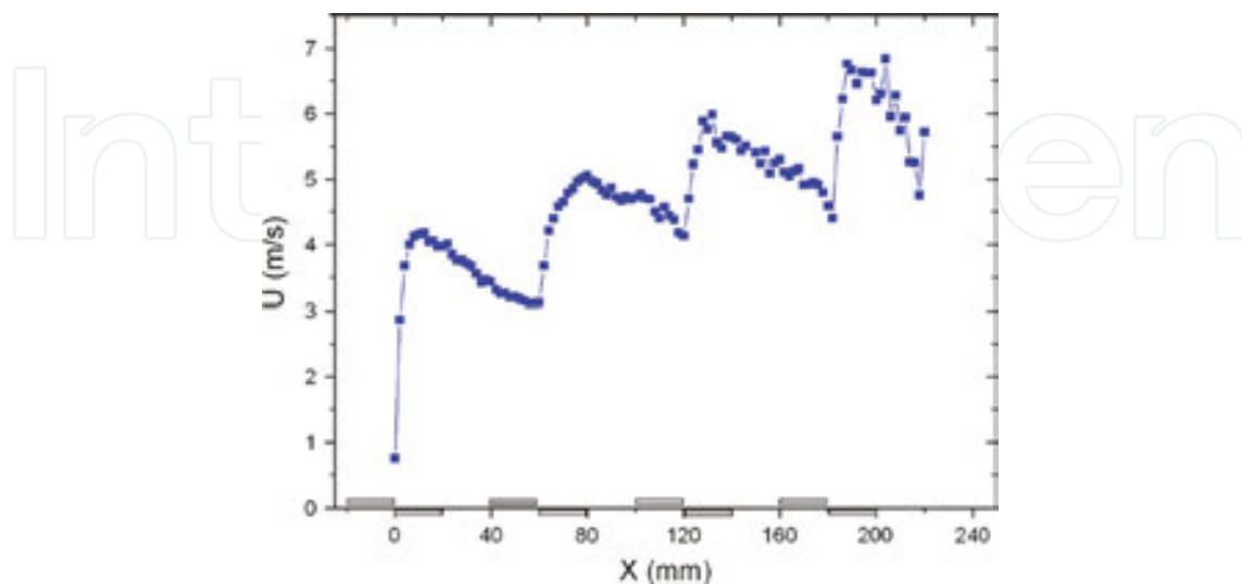
Figure 7. Horizontal velocity profile ( y = 0.5 mm) above four DBD actuators in series [13].
