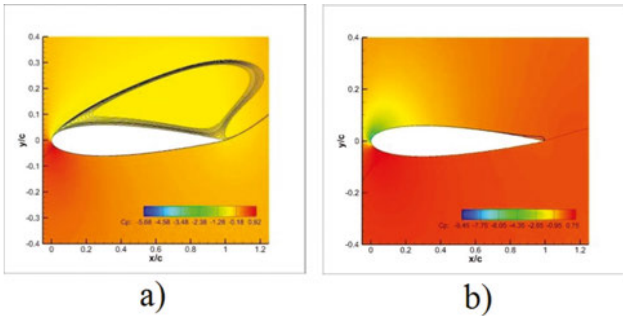
Figure 16. Pressure coefficient contours with streamlines over an airfoil with 15° angle of attack: plasma actuator off (a) and on (b) [47].
