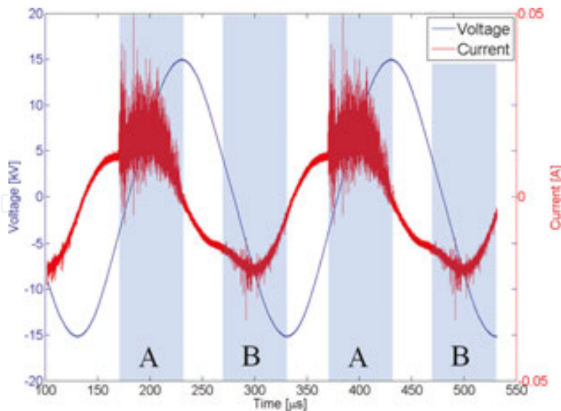
Figure 3. Voltage-current time behavior of a SDBD [15].
