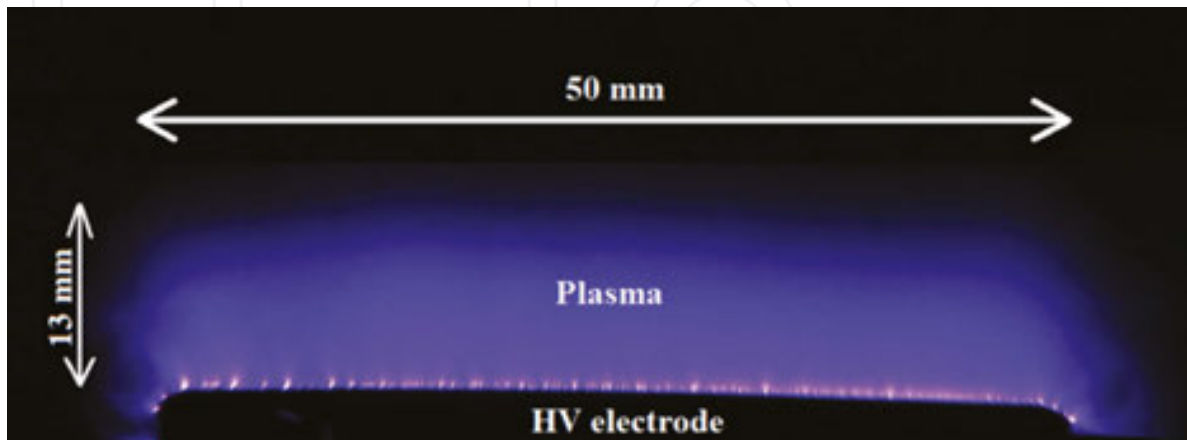
Figure 2. Top view image of SDBD discharge [14].
