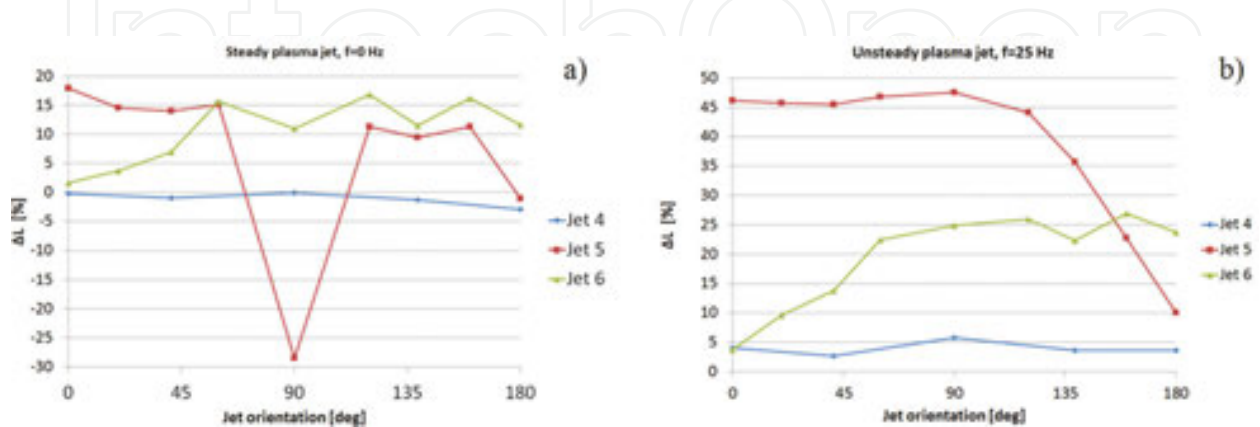
Figure 17. Lift recovery in percentage for different actuators location with a free stream velocity of 11 m/s: steady operation (a) and duty cycle operation (b) [66].
