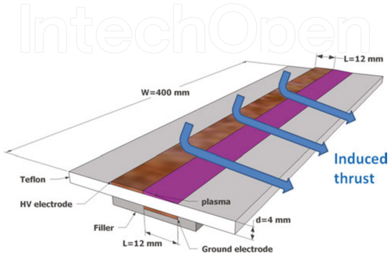
Figure 1. Schematic of a SDBD actuator for flow control.
