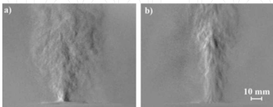
Figure 11. Schlieren images of PSJAs of linear (a) and annular (b) geometries. Electrode distance (a) and diameter (b) is 30 mm.
