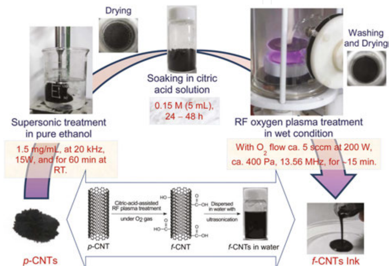
Figure 3. The flow chart of the functionalization process with the optimum treatment conditions and the schematic of the functional group attachment.
