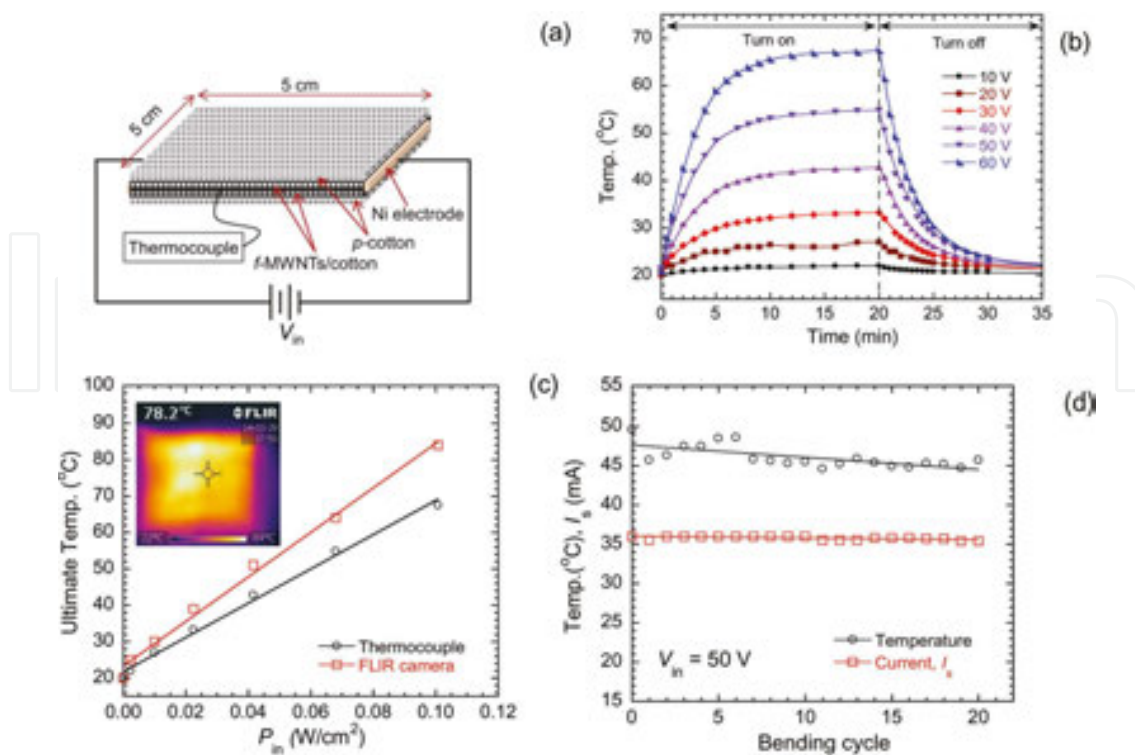
Figure 12. Heating and cooling temperatures of the f -CNTs/ cotton textile of R_s = 1.67 k \Omega /sq using a dc power supply. (a) Schematic of the heat measurement setup. (b) Heating and cooling temperatures at the center of the textile with time measured by a thermocouple. (c) The increase in ultimate temperature of the f -CNTs/cotton textile with input power (inset: thermal image at V_{in} = 60 V showing the uniform heating of the textile). (d) Changes in the temperature and current after repeated bending.
