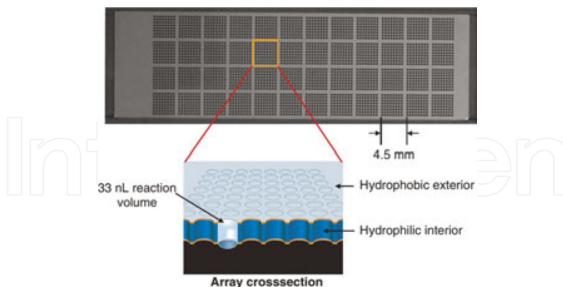
Figure 2. Plate-based chip used for the OpenArray RealTime PCR System. A rectilinear array of 3072 microholes with 320 \mu\text{m} in diameter was fabricated in a stainless steel plate (25 \times 75 \times 0.3 mm). The volume of each hole was approximately 33 nanoliters, and to match the pitch of the wells in a 384-well microplate, the 48 groups of 64 holes are spaced at 4.5 mm. Reprinted with permission from Ref. [43]. © Copyright 2006 Oxford University Press.
