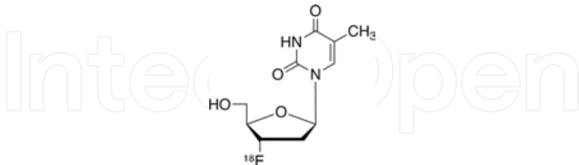
Figure 8. Chemical structure of F-18 fluorothymidine.
